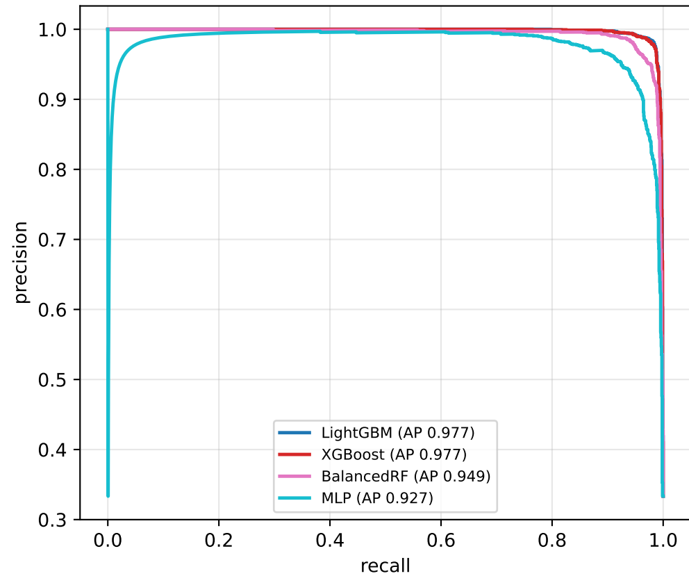
Precision-recall (micro-average)
