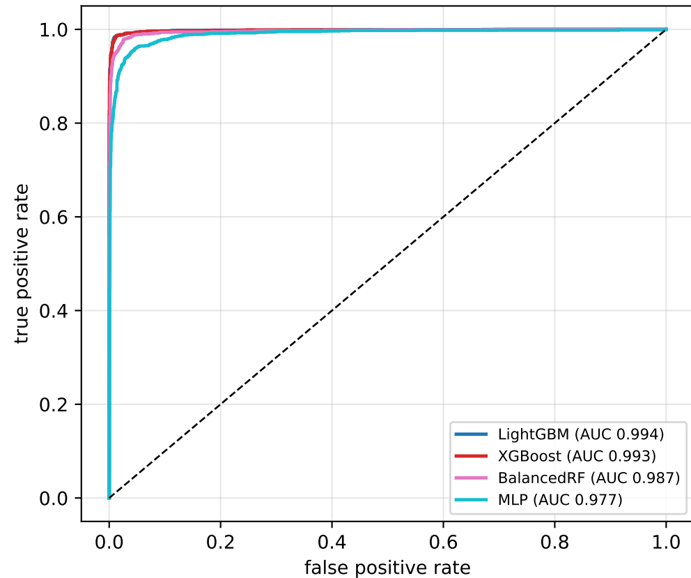
ROC (micro-average)
