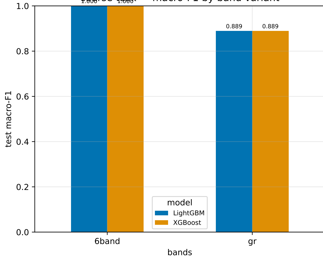
coarse task — macro-F1 by band variant
