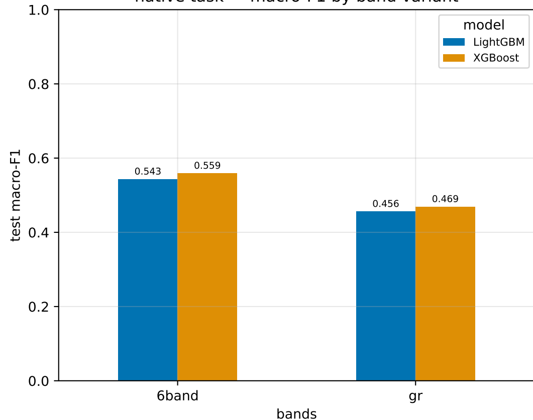
native task — macro-F1 by band variant
