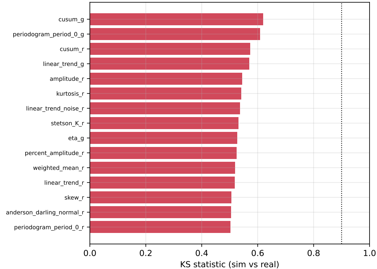
A_normalised: 15 most domain-separated features
