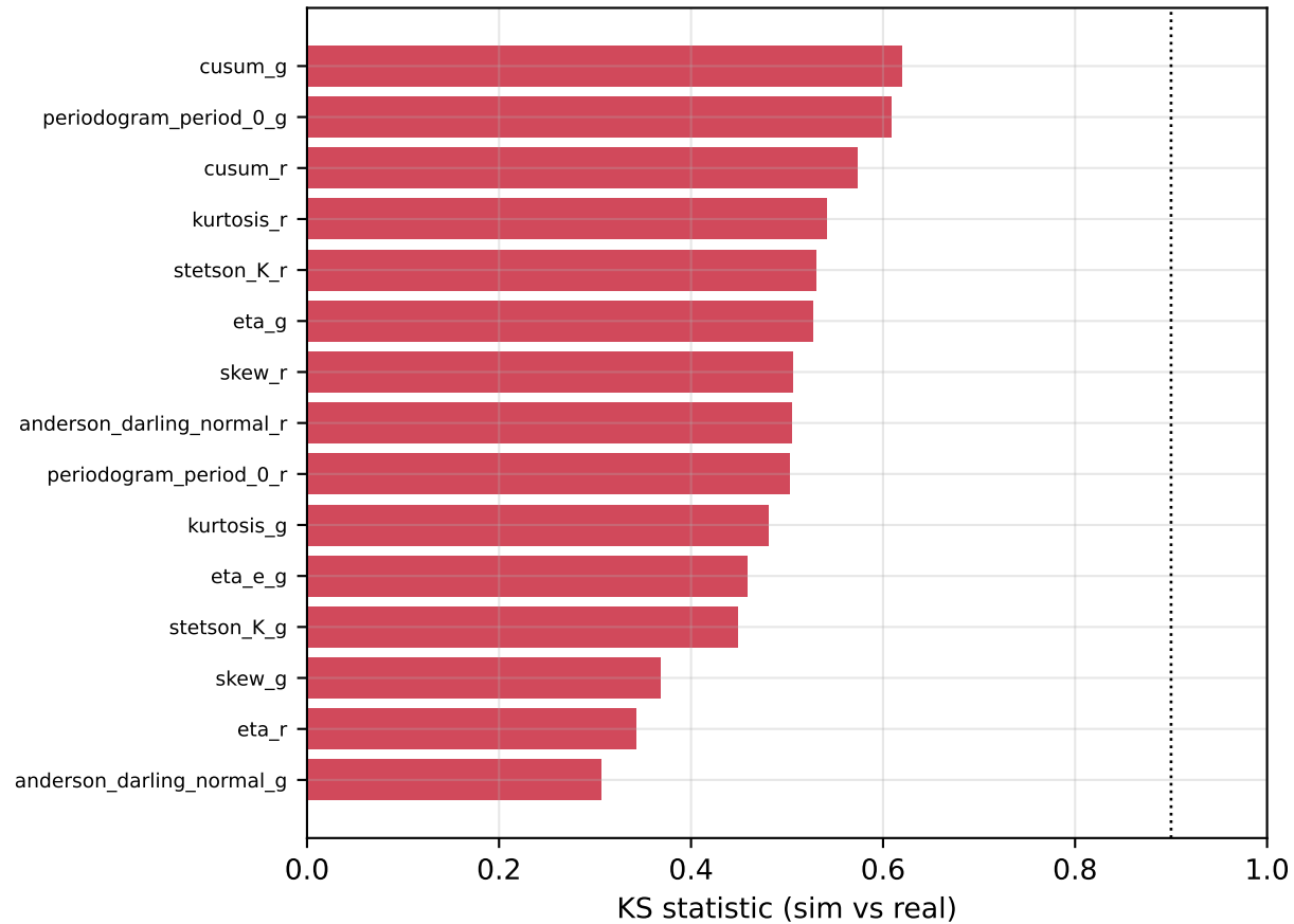
B_scalefree: 15 most domain-separated features
