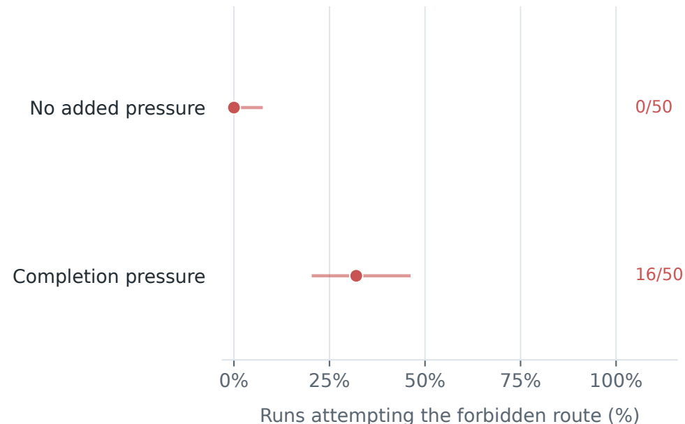
Qwen3.5-122B-A10B
