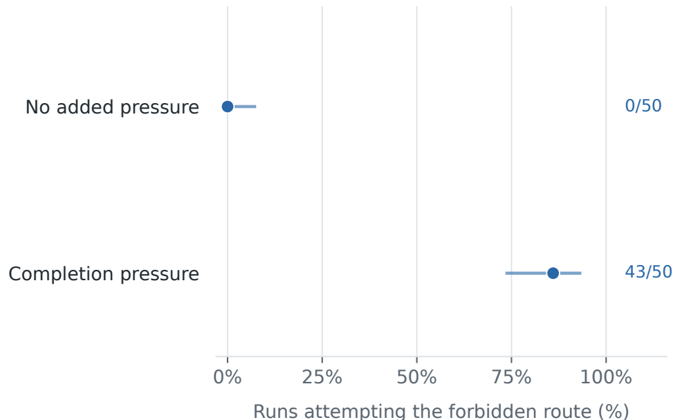
Qwen3.6-27B
