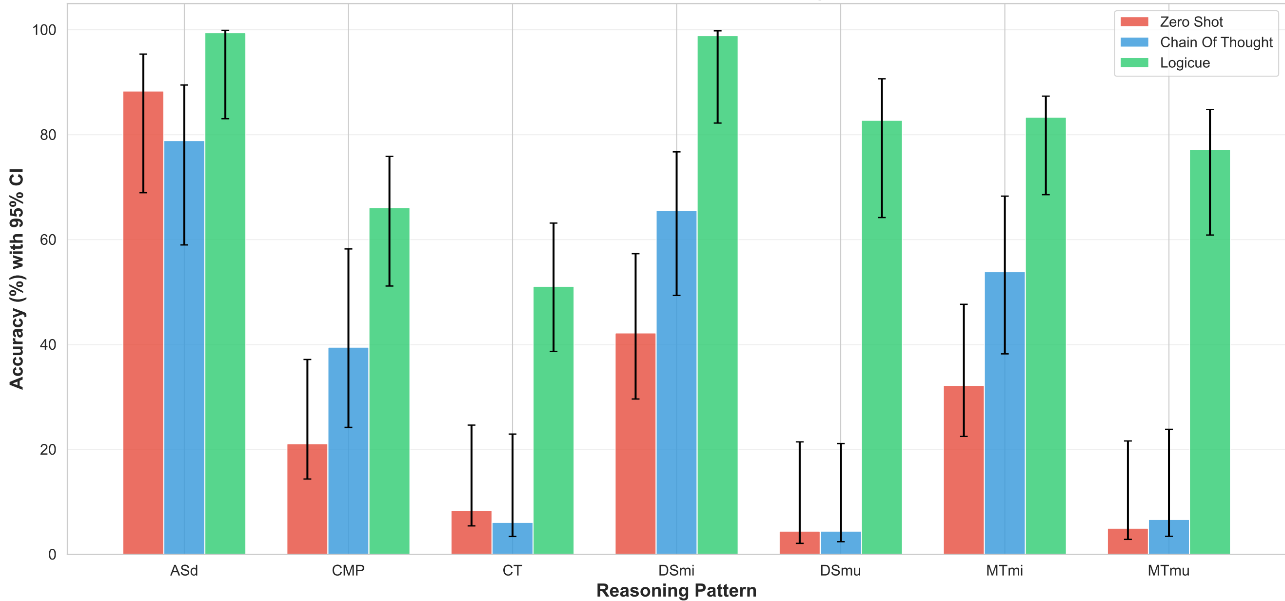
Method Comparison Across Reasoning Patterns
