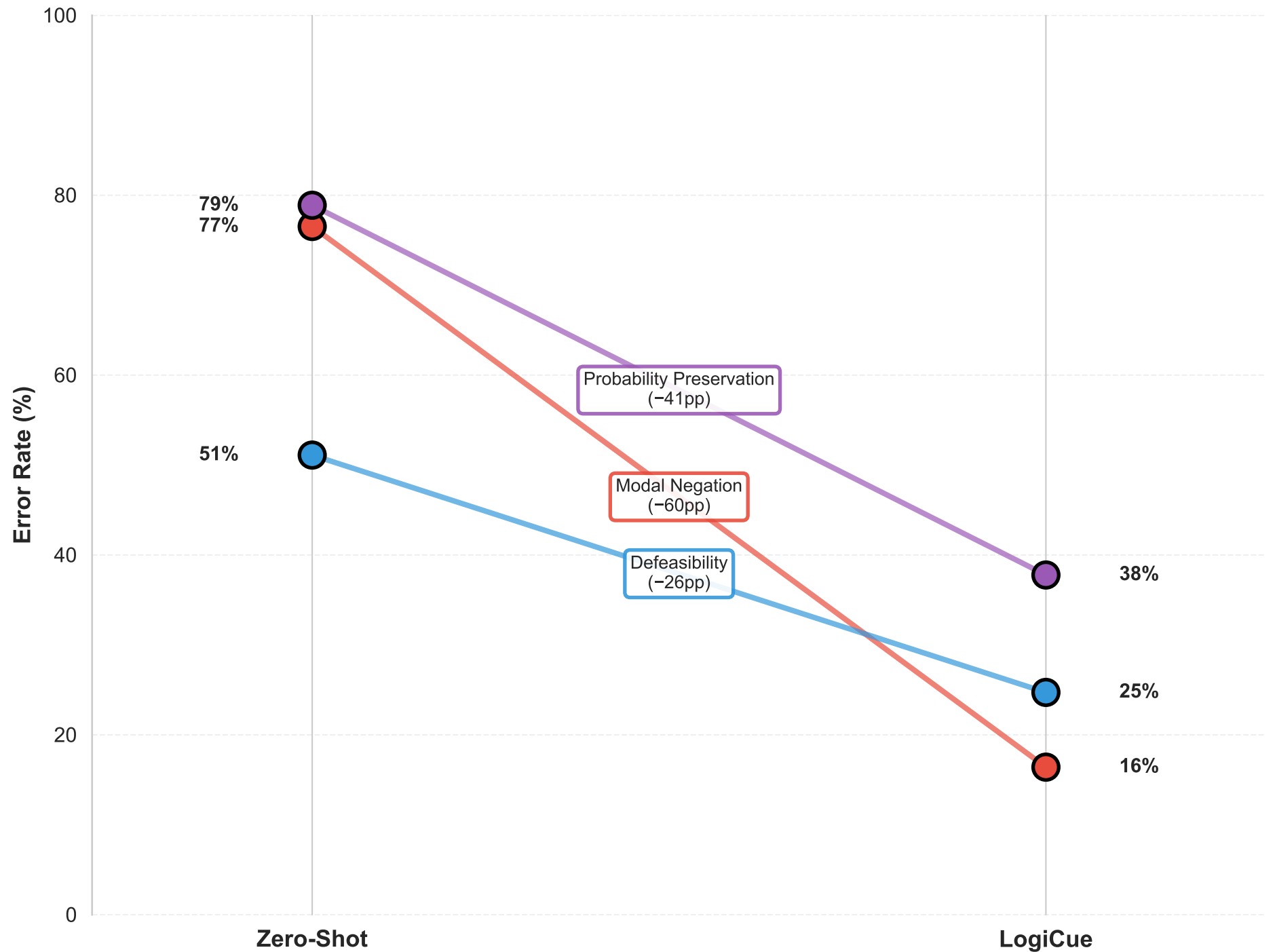
Error Rate Reduction by Category: Zero-Shot → LogiCue
