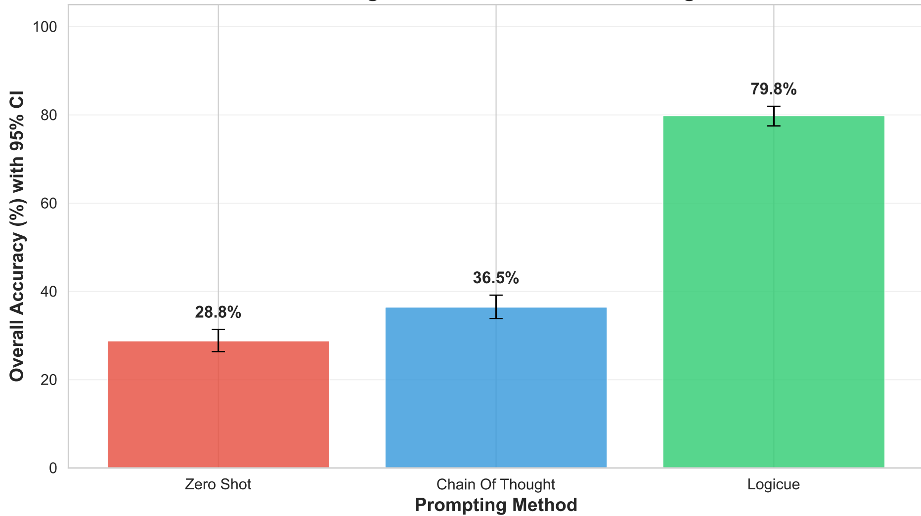
Method Progression: From Zero-Shot to LogiCue
