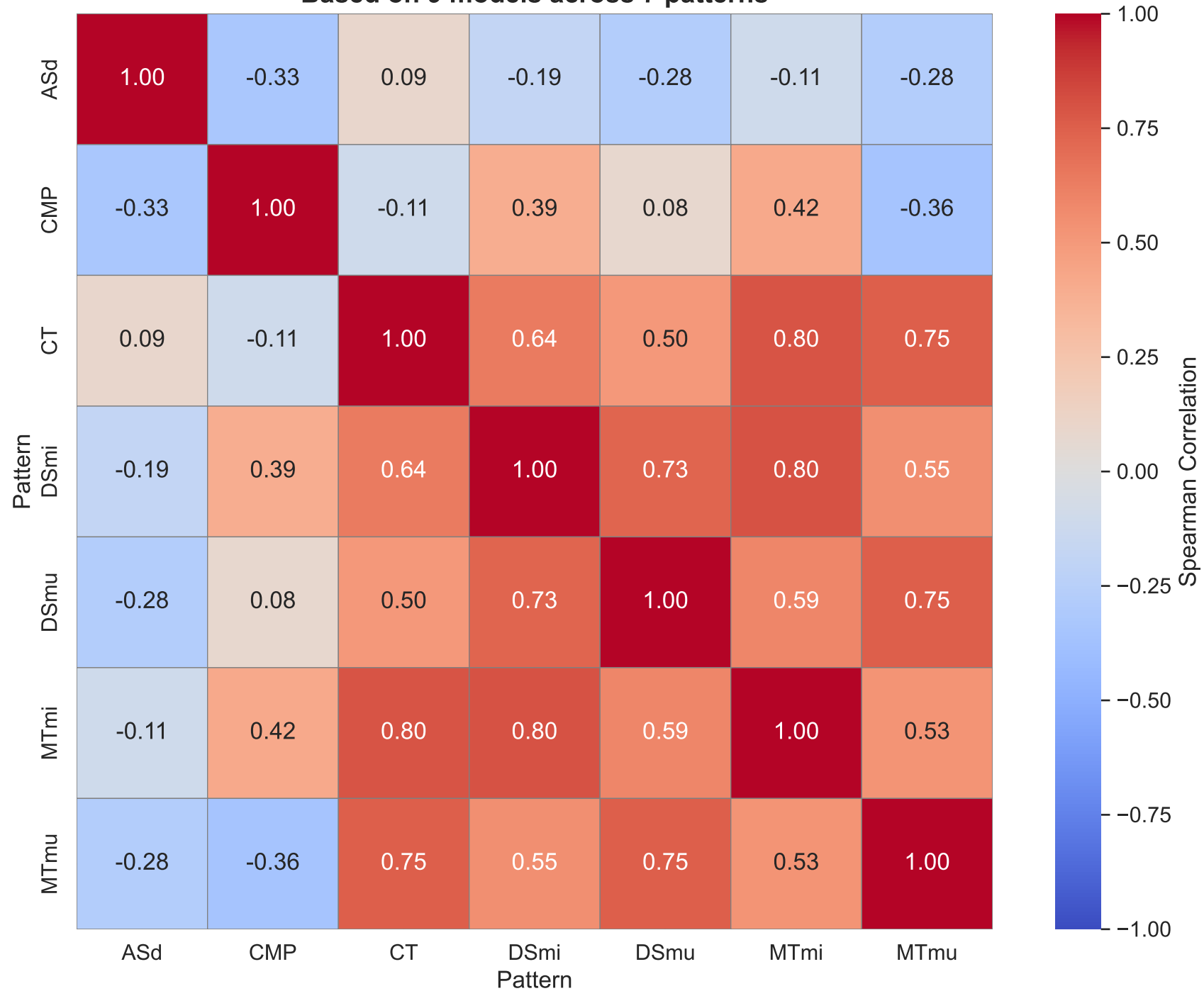
Cross-Pattern Correlation Analysis (Zero-Shot) Based on 9 models across 7 patterns
