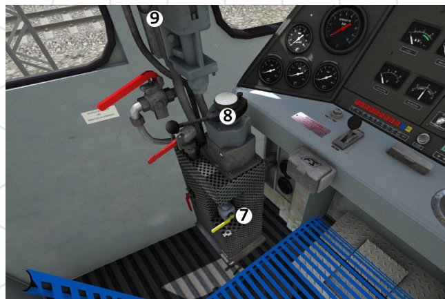
Figure 4 — Isolating cock (7), train brake (8), loco brake (9)
