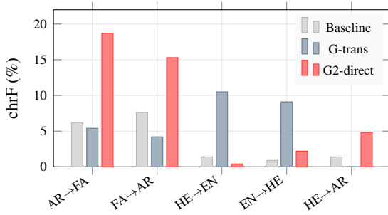
Figure 3: Translation tradeoff. EN-mediated helps EN \leftrightarrow X ; direct parallel needed for X \leftrightarrow Y .
