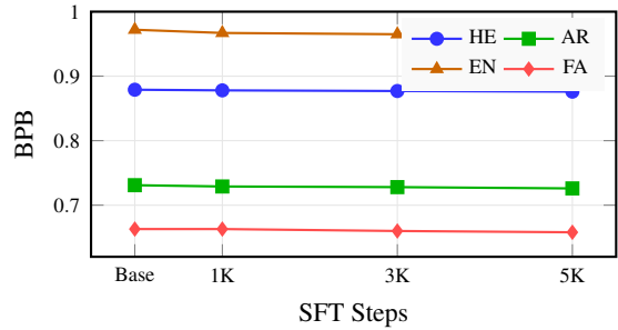
Figure 2: BPB improvement with SFT scaling. Diminishing returns after 3K steps.
