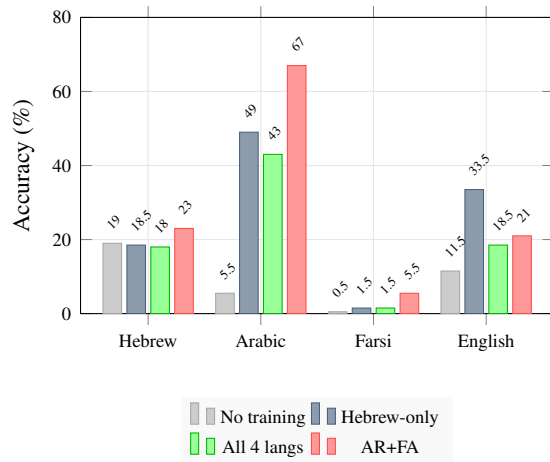
Figure 5: Cross-lingual sentiment transfer. Hebrew-only (blue) improves Arabic 9× with zero Arabic data. Farsi shows no transfer despite shared script.
