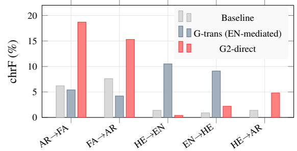
Figure 3: Translation strategy tradeoff. G-trans (English-mediated) helps EN↔X but fails for direct X↔Y. G2-direct excels at trained pairs but collapses EN↔X. Practitioners must choose based on their target pairs.
