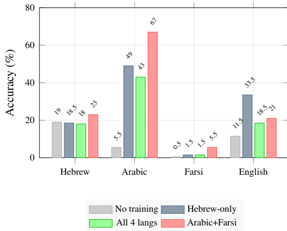
Figure 5: Cross-lingual sentiment transfer results. The Hebrew-only configuration (navy) improves Arabic from 5.5% to 49% (9×) despite receiving zero Arabic sentiment data. Farsi (same script as Arabic, Indo-European family) shows no transfer—confirming that linguistic family, not script, drives transfer .
