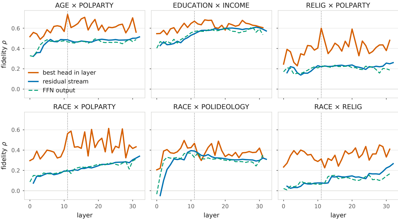
Attention heads dominate the residual stream at every depth
