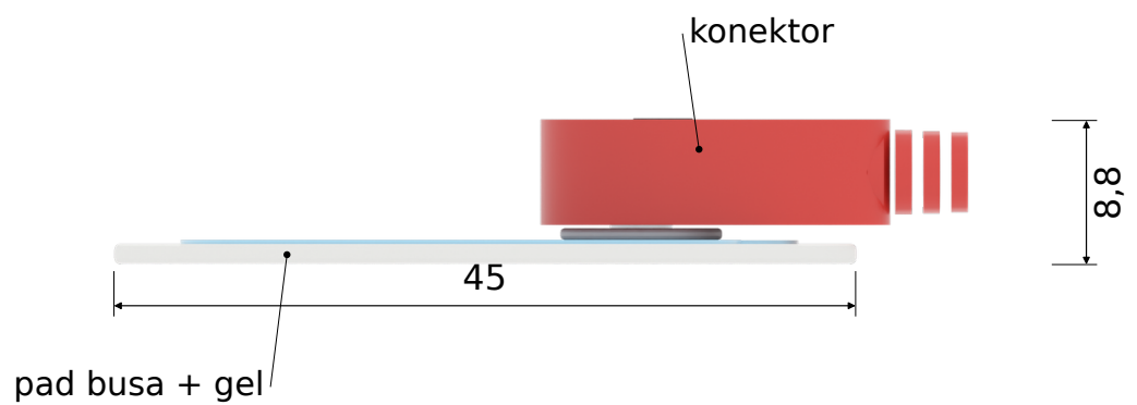
C. Tampak samping (mm)
