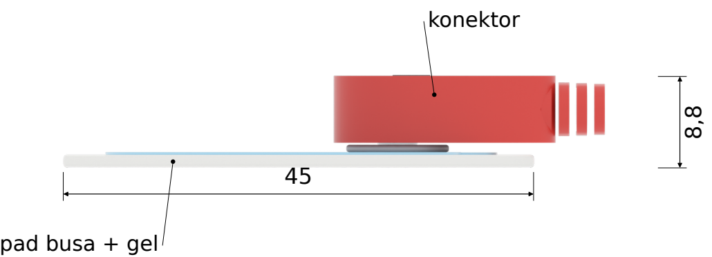
C. Tampak samping (mm)
