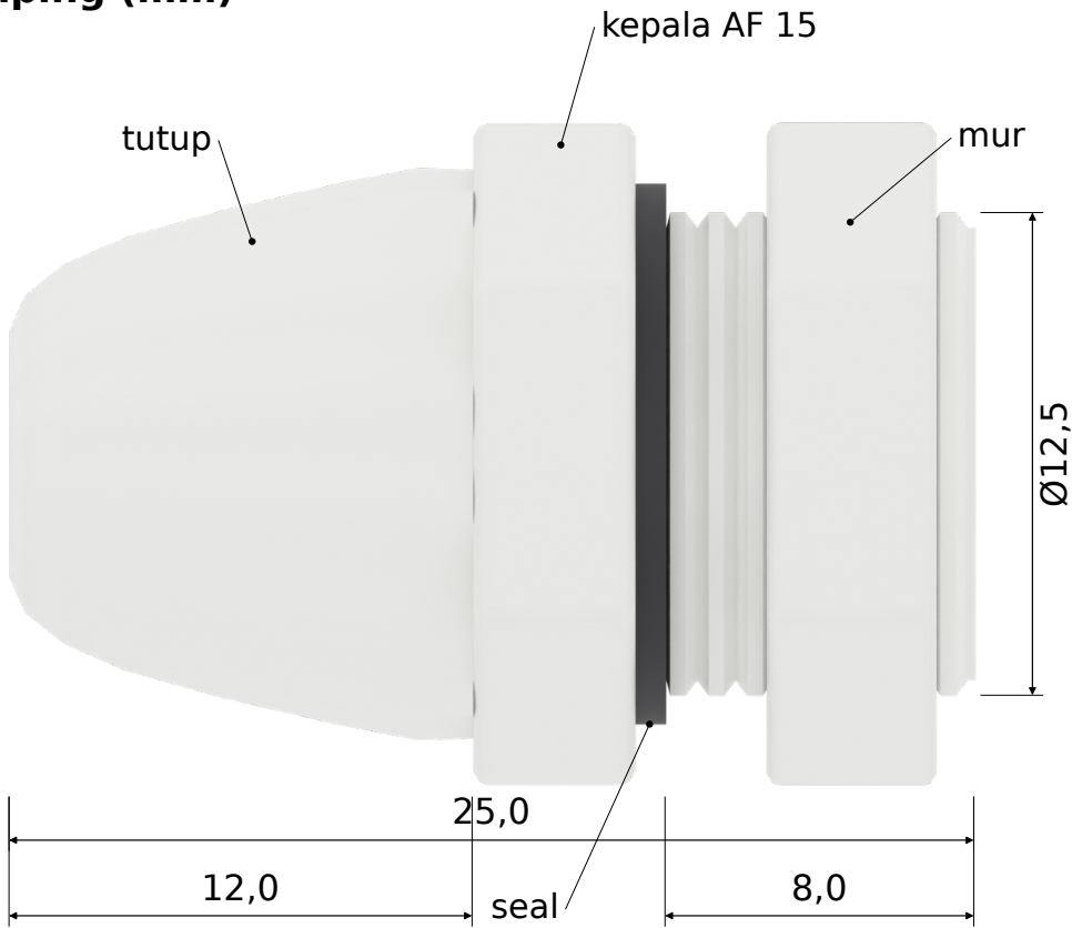
B. Tampak samping (mm)
