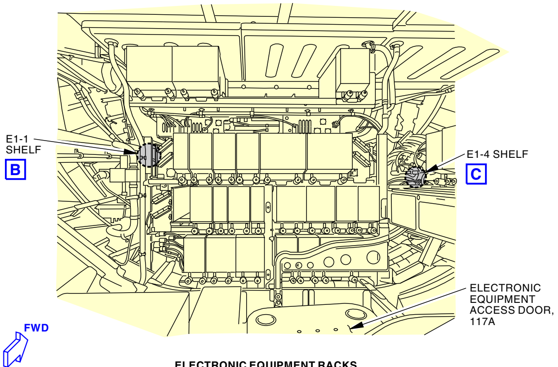
ELECTRONIC EQUIPMENT RACKS
