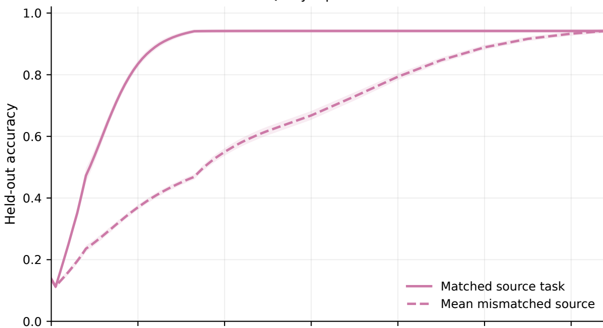
Key-input Gram
