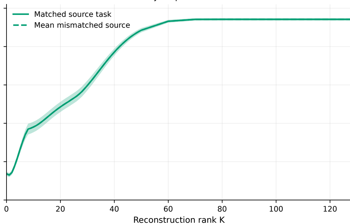
Key-output Gram
