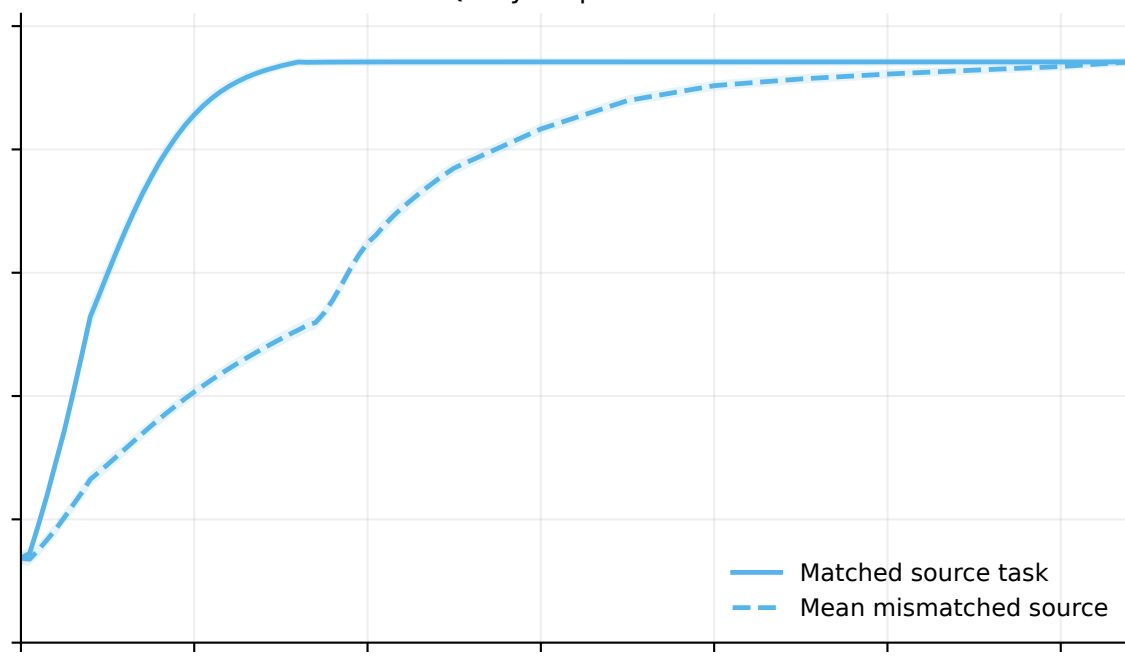
Key-output Gram
