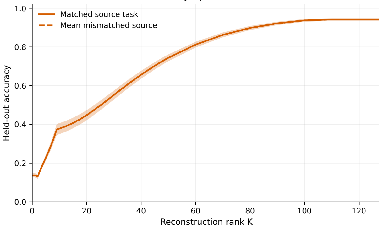
Key-input Gram
