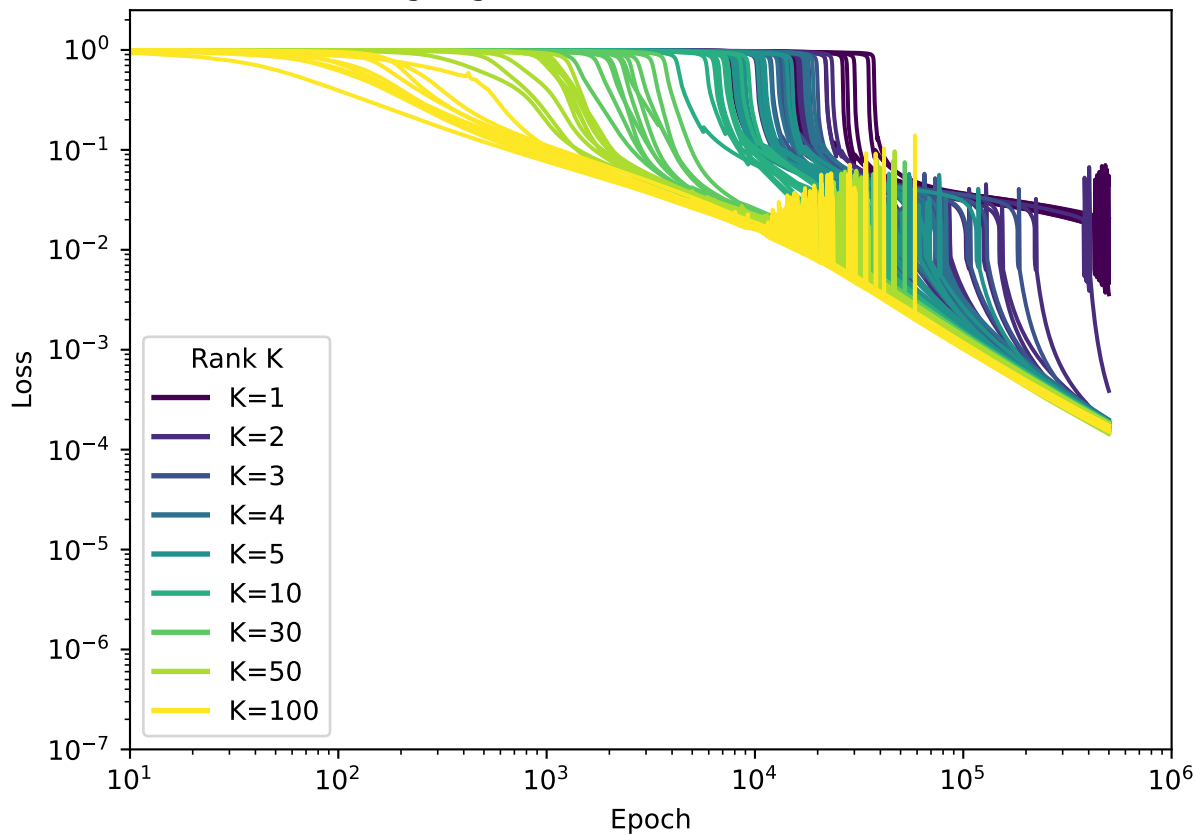
log-log loss curves ( \text{lr} = 1.00\text{e-}03 )
