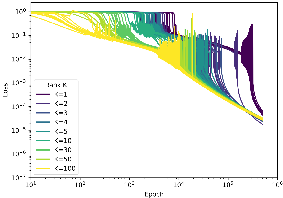
log-log loss curves ( \text{lr} = 4.64\text{e-}03 )
