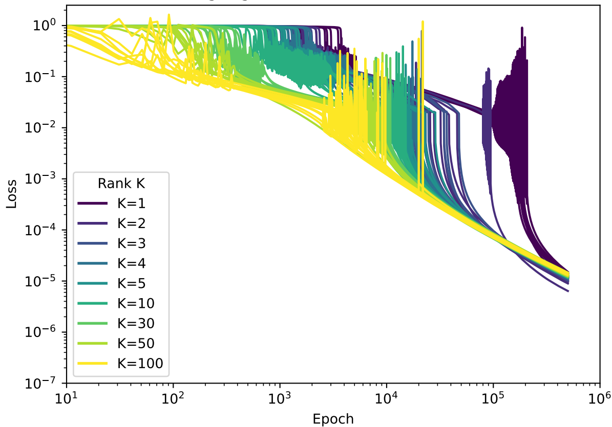
log-log loss curves ( \text{lr} = 1.00\text{e-}02 )
