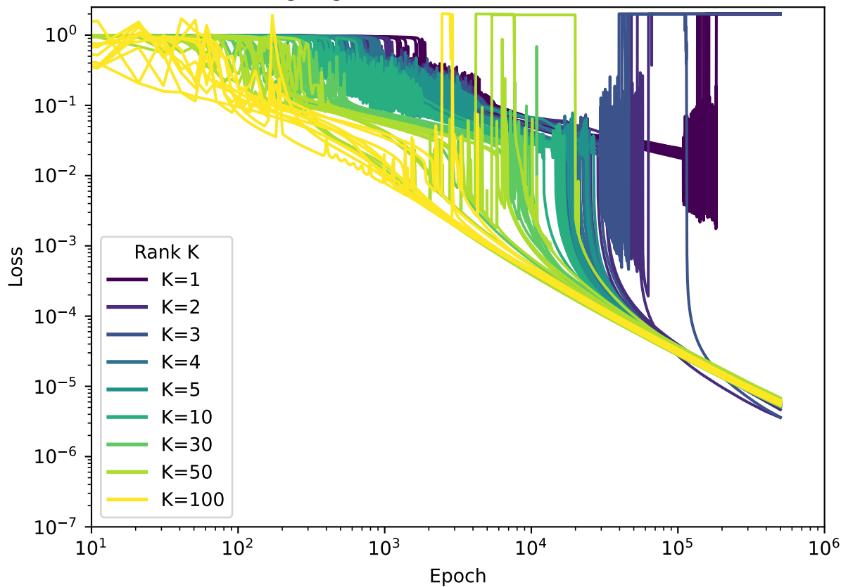
log-log loss curves (lr = 2.15e-02)
