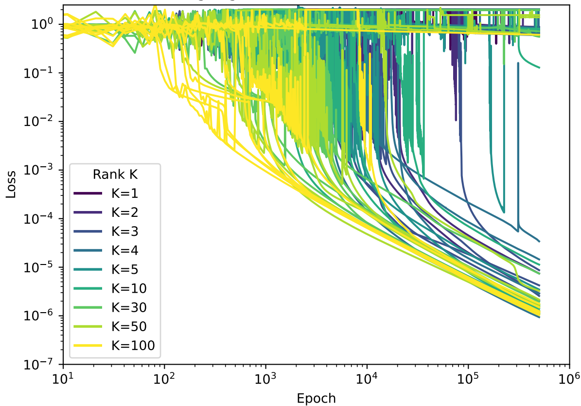
log-log loss curves ( \text{lr} = 1.00\text{e-}01 )
