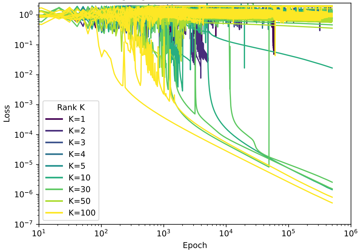
log-log loss curves ( \text{lr} = 2.15\text{e-}01 )
