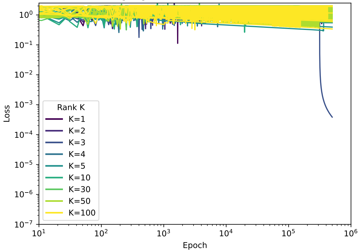
log-log loss curves ( \text{lr} = 4.64\text{e-}01 )
