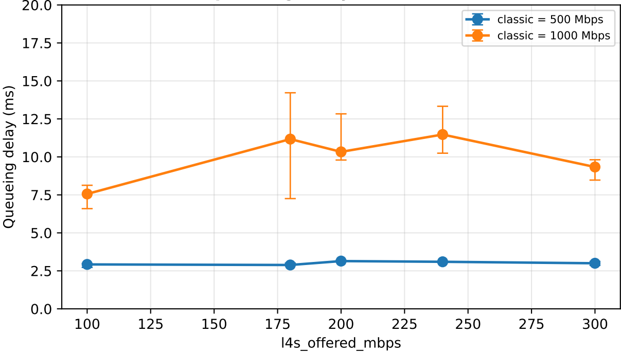
Classic queueing delay (base RTT = 30 ms)
