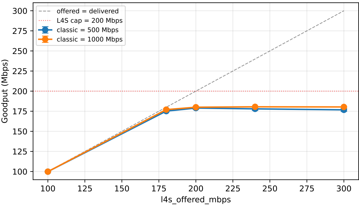
L4S goodput
