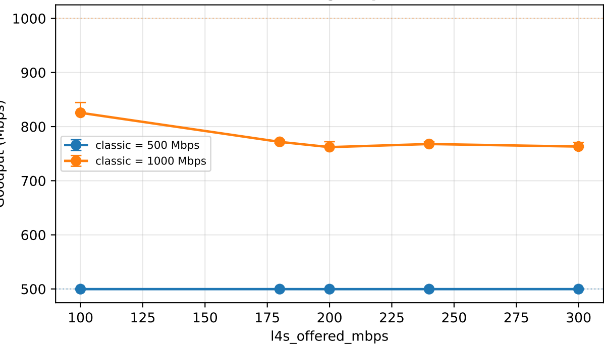
Classic goodput
