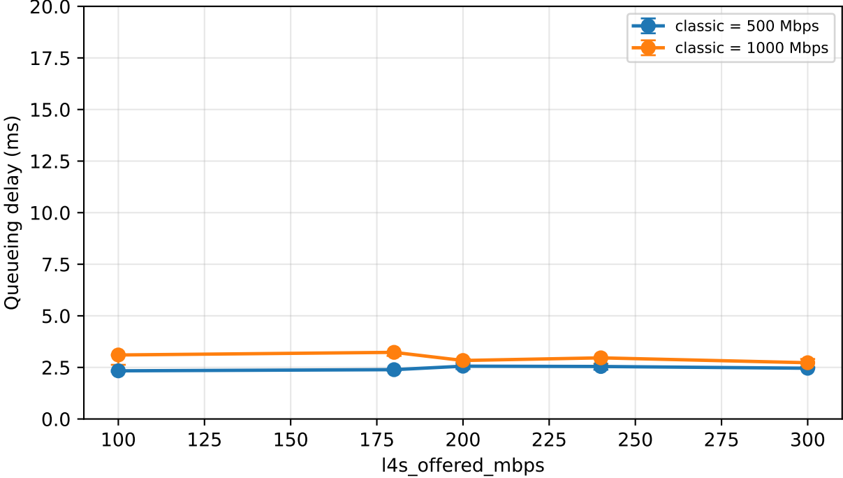
L4S queueing delay (base RTT = 30 ms)
