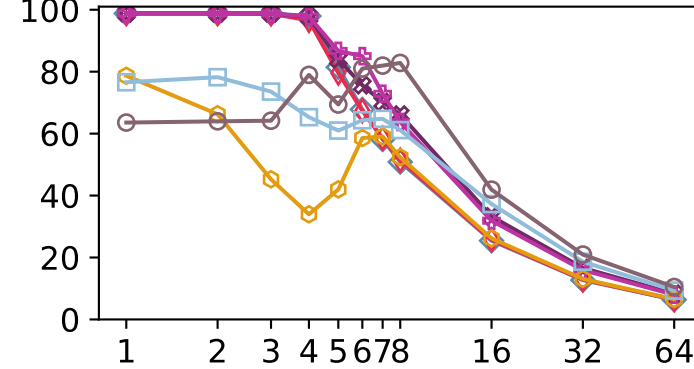
Buffer Occupancy [%]
