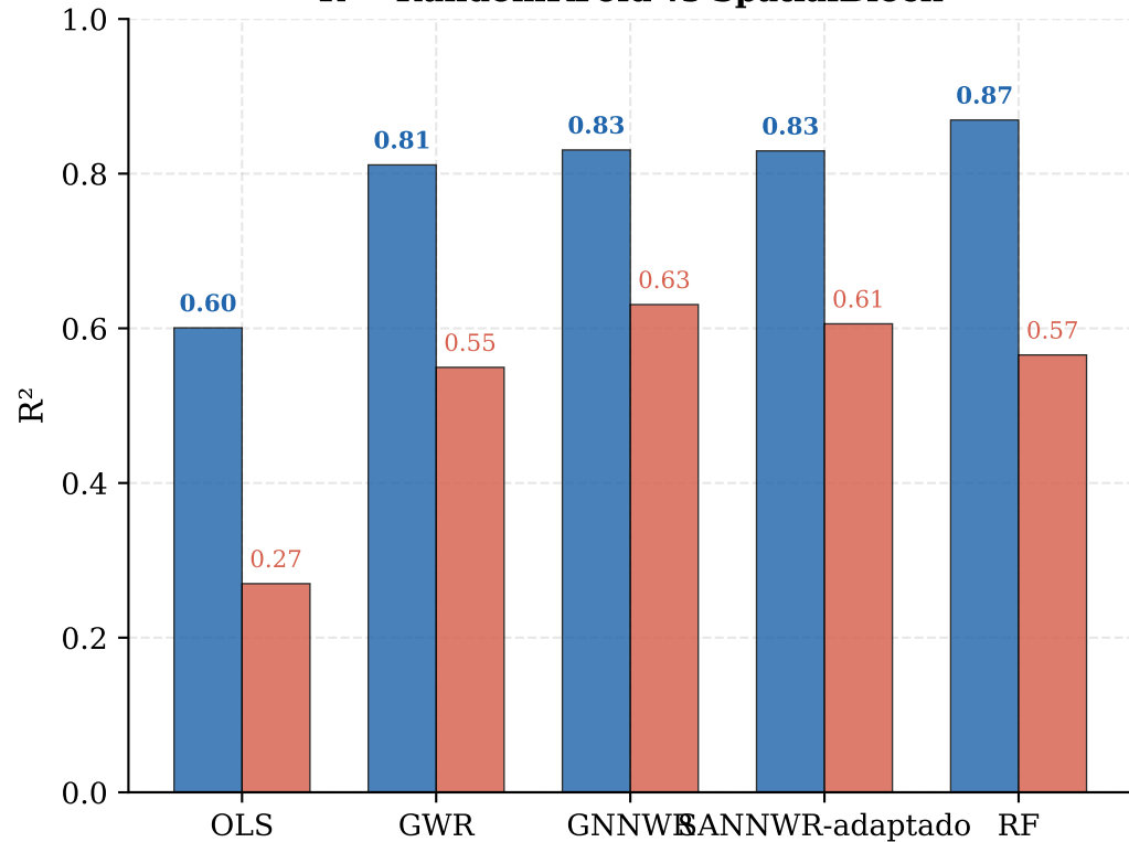
R² - RandomKFold vs SpatialBlock
