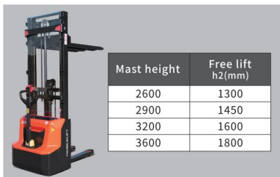
Full Free Mast Structure
