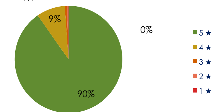
Rating Distribution
