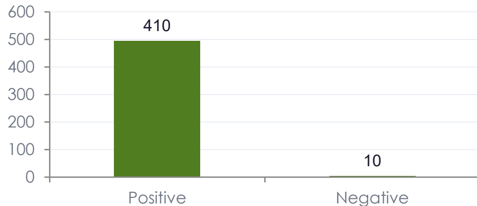
Sentiment Distribution
