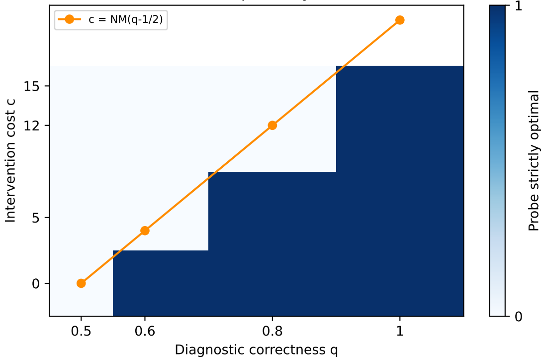
One-intervention optimality ( N=4 , M=10 )
