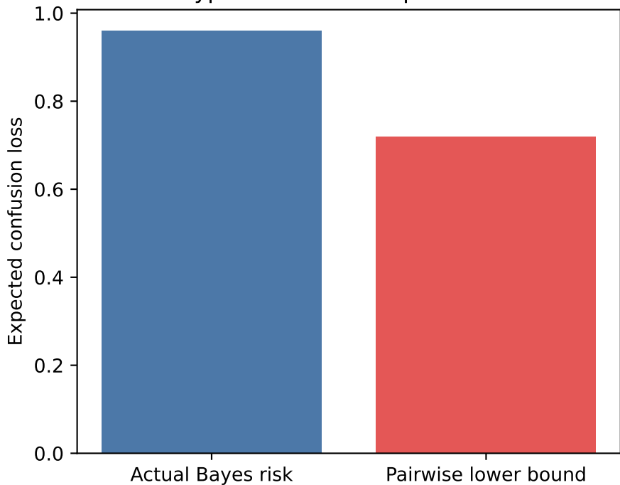
Multi-type risk and valid pairwise bound
