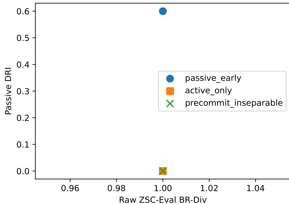
Matched best-response diversity does not determine timely DRI
