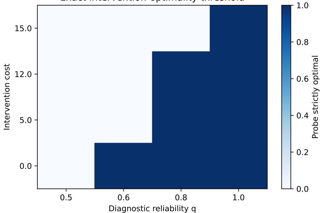
Exact intervention-optimality threshold
