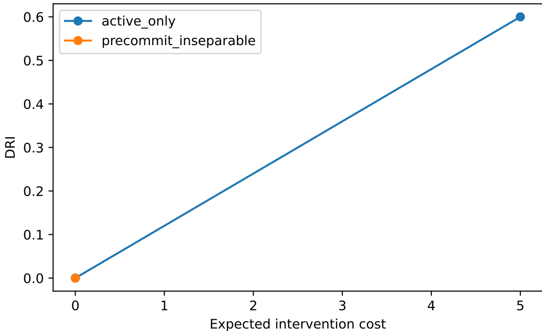
Matched active-identifiability frontiers
