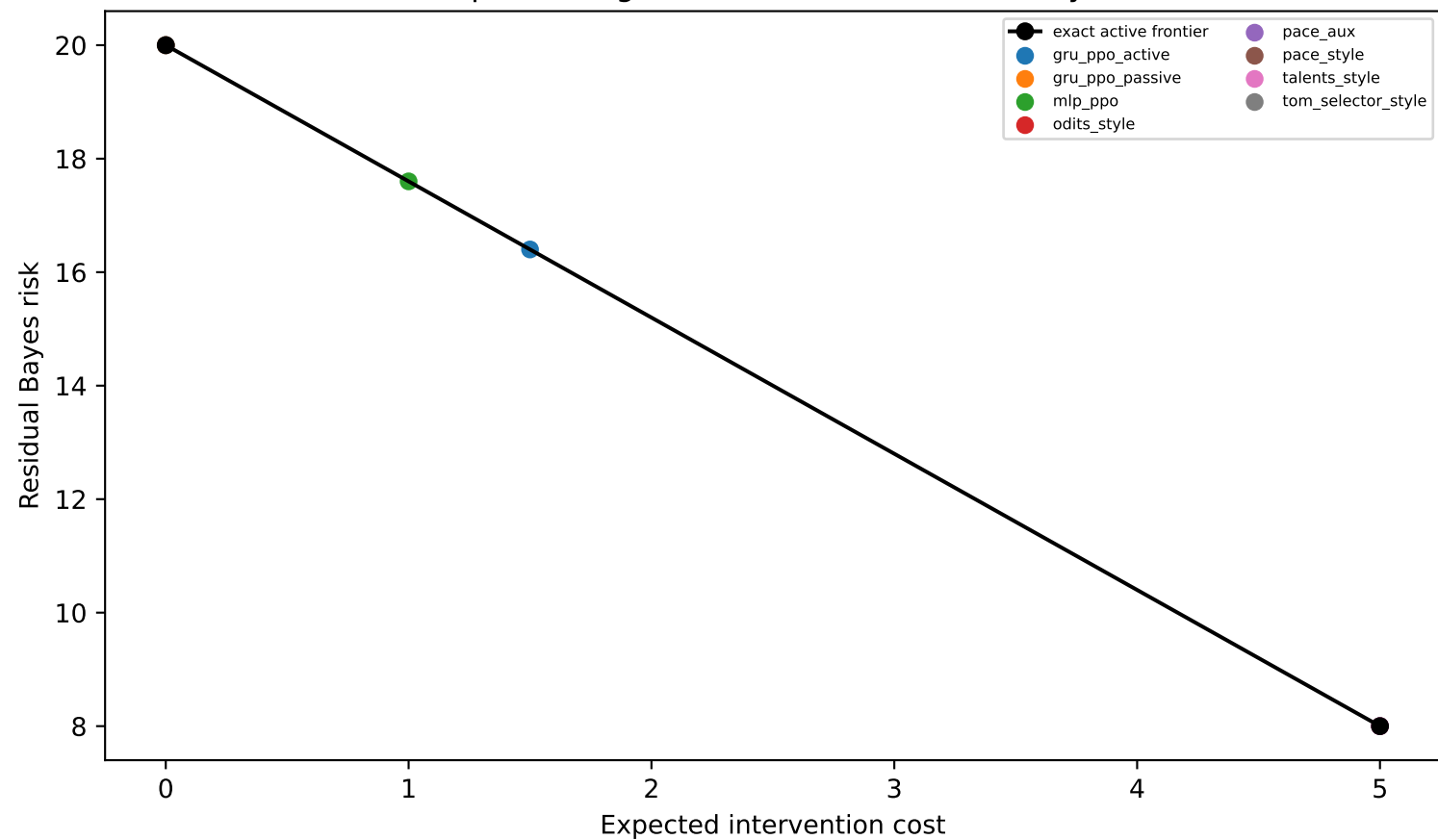
Learned policies against the active-identifiability frontier
