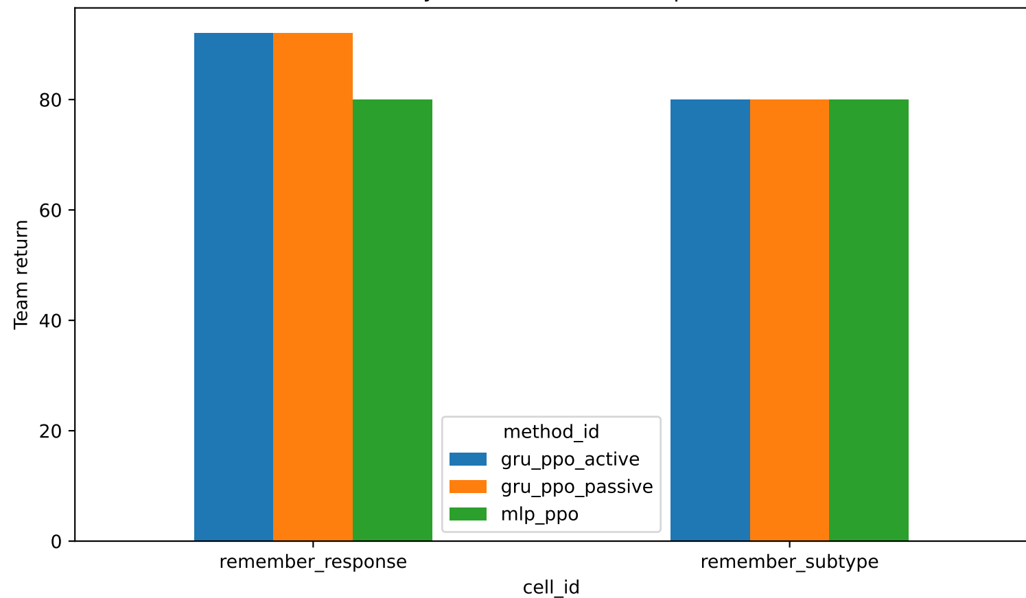
Memoryless versus recurrent policies
