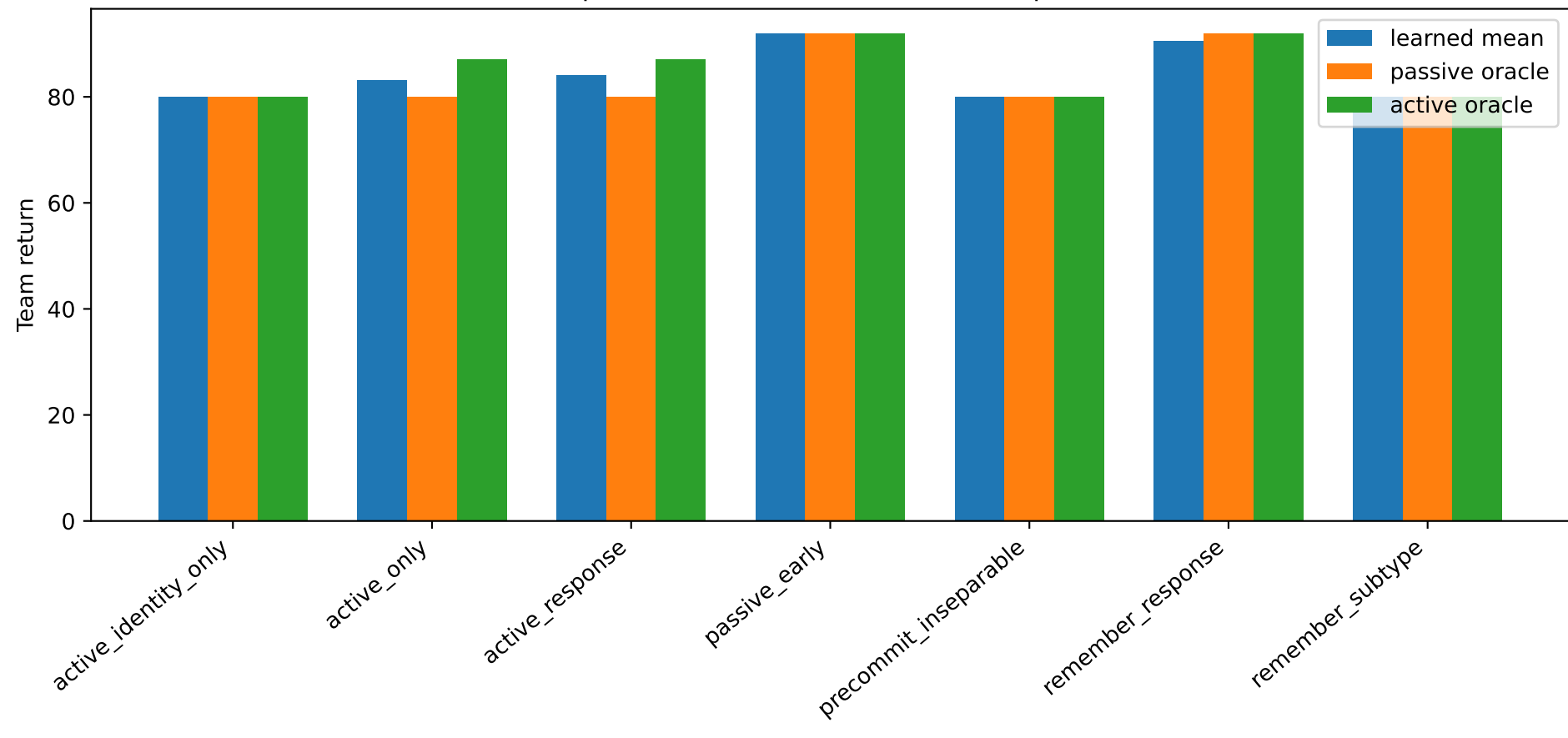
Learned, passive-oracle, and active-oracle performance
