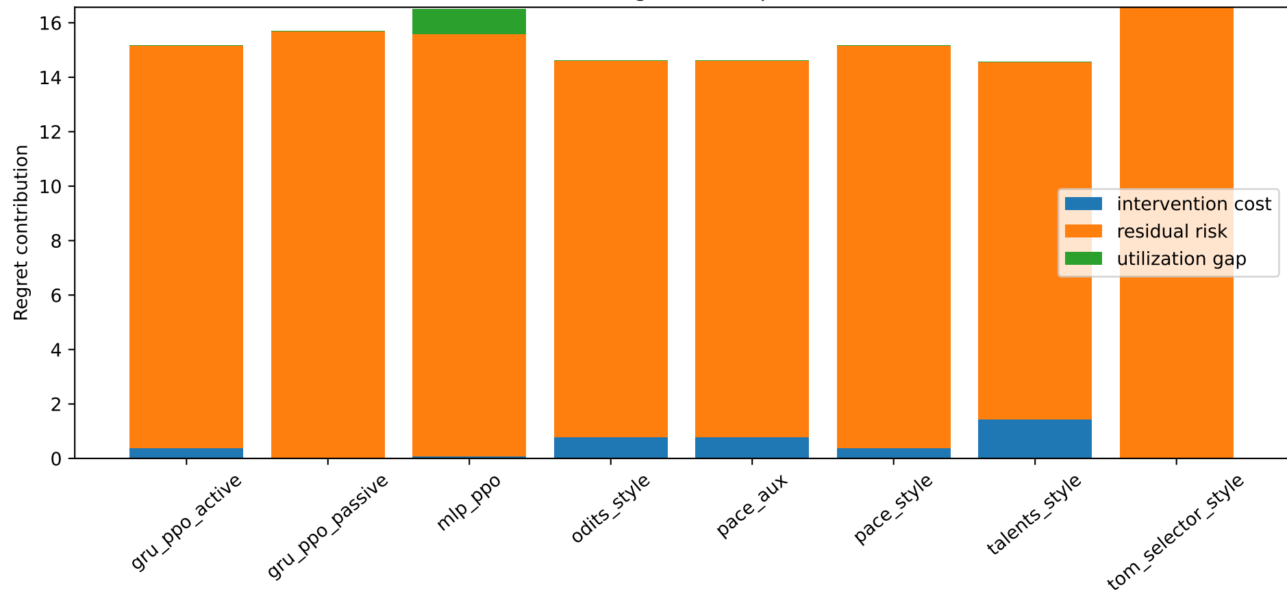
Learned regret decomposition
