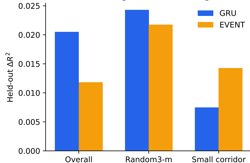
Predictive gain from adding DRI
