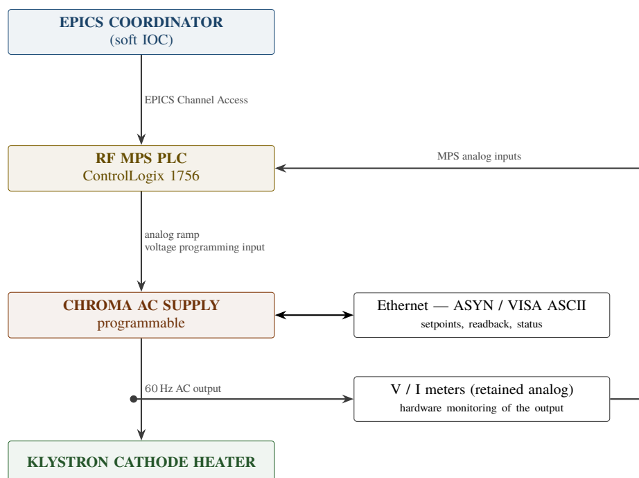
Figure 5: Klystron cathode heater controller architecture. Three paths are deliberately separate: the MPS ramps the Chroma output through the analog programming input, so controlled warm-up and cooldown do not depend on the network; the Ethernet link carries setpoints and readback only; and the existing analog V/I meters are retained, so the delivered output is monitored in hardware independently of both. There are no mechanical components anywhere in the control path.
