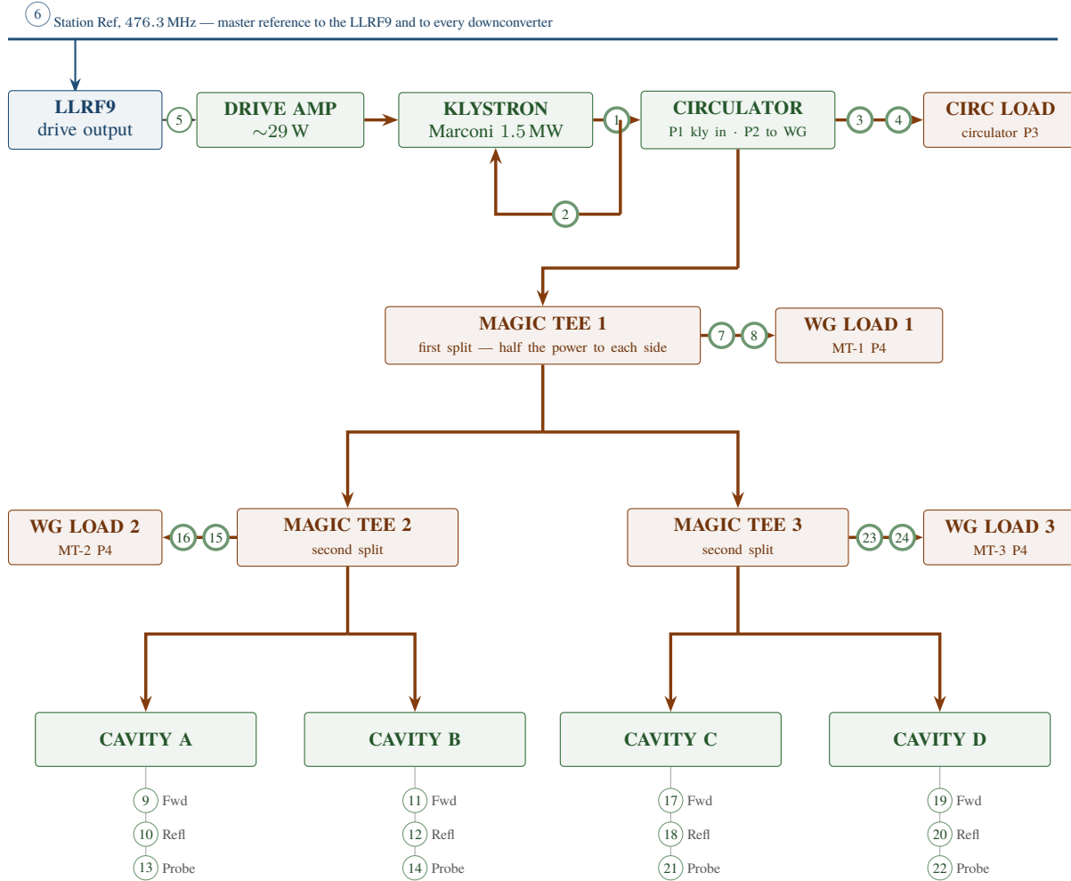
Figure 2: RF plant signal flow. Heavy lines are waveguide, light lines coaxial. Circled numbers are the directional-coupler channel indices used in Section 4.6.
