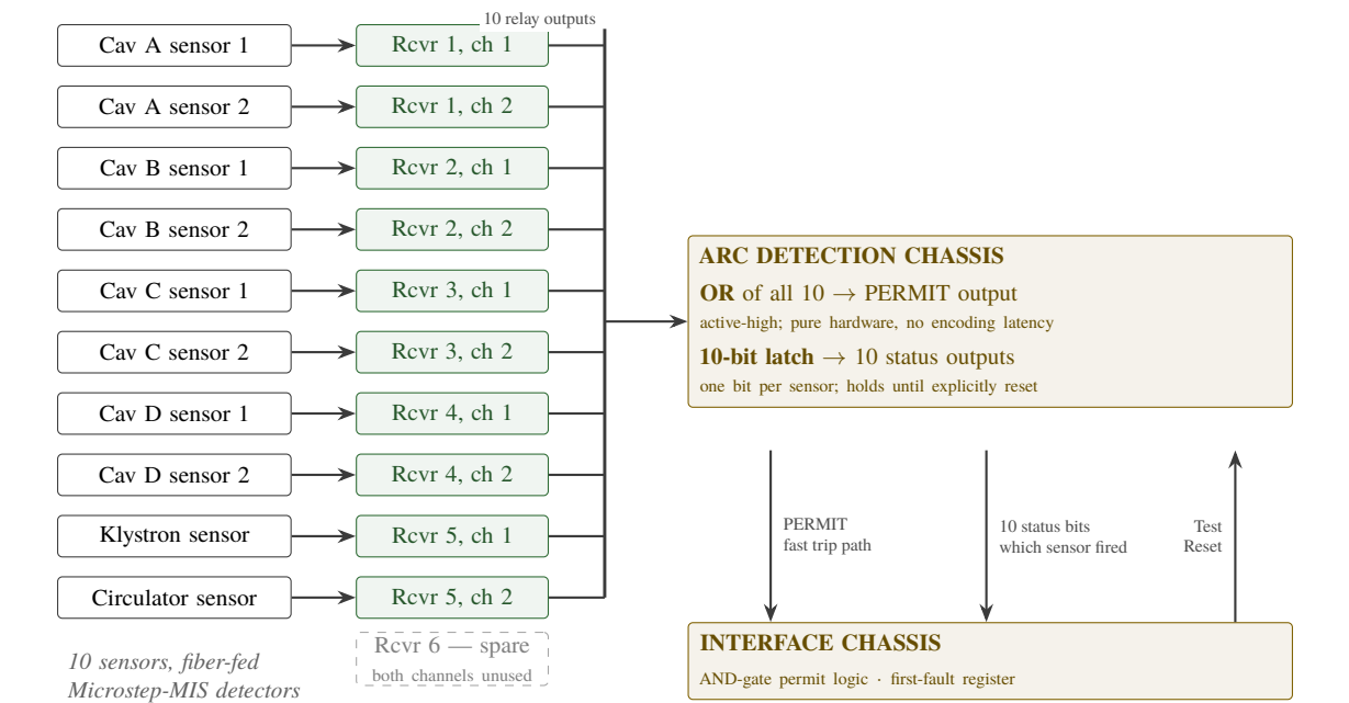
Figure 4: Arc detection signal path. The two outputs run in parallel: an all-hardware OR gives the fast trip, while the 10-bit latch preserves which sensor fired for post-mortem analysis.
