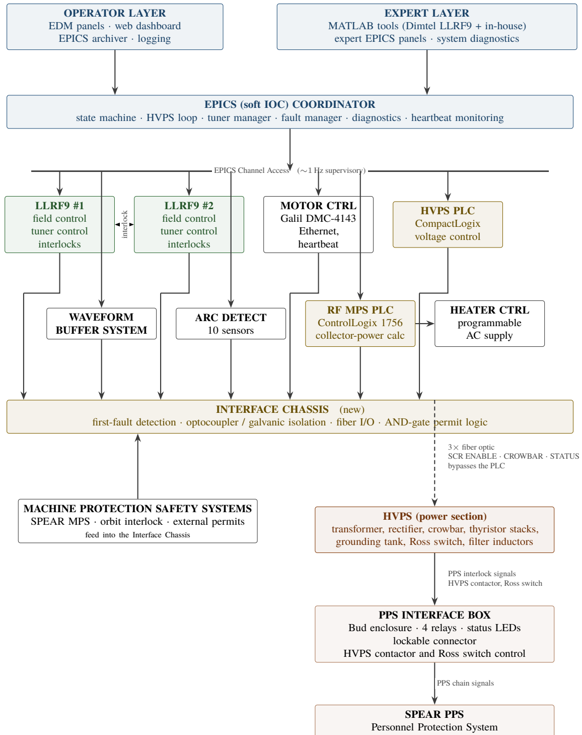
Figure 1: Upgraded system architecture. The Interface Chassis is the single hub for machine and equipment protection; personnel safety runs on a physically and logically separate path through the PPS Interface Box to the SPEAR PPS.
