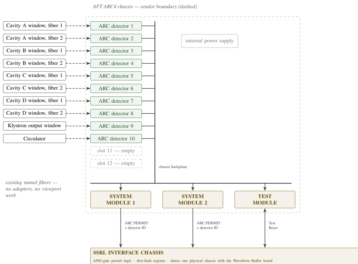
Figure 4: Arc detection signal path. The dashed outline is the vendor boundary: everything inside it is AFT ARC4 hardware, and no SSRL wire lands on an individual detector module. Fibers enter the detector modules from the front; the detector modules drive the chassis backplane; only the two system modules and the test module face the Interface Chassis. Ten of the chassis’s twelve slots are populated; slots 11 and 12 are left empty and their two detector modules are held as shelf spares.
