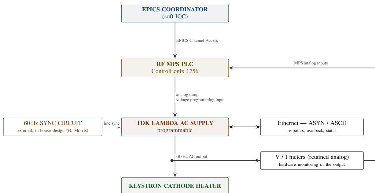
Figure 5: Klystron cathode heater controller architecture. Three paths are deliberately separate: the MPS ramps the TDK Lambda output through the analog programming input, so controlled warm-up and cooldown do not depend on the network; the Ethernet link carries setpoints and readback only; and the existing analog V/I meters are retained, so the delivered output is monitored in hardware independently of both. The external 60 Hz sync circuit is a new in-house design item. There are no mechanical components anywhere in the control path.
