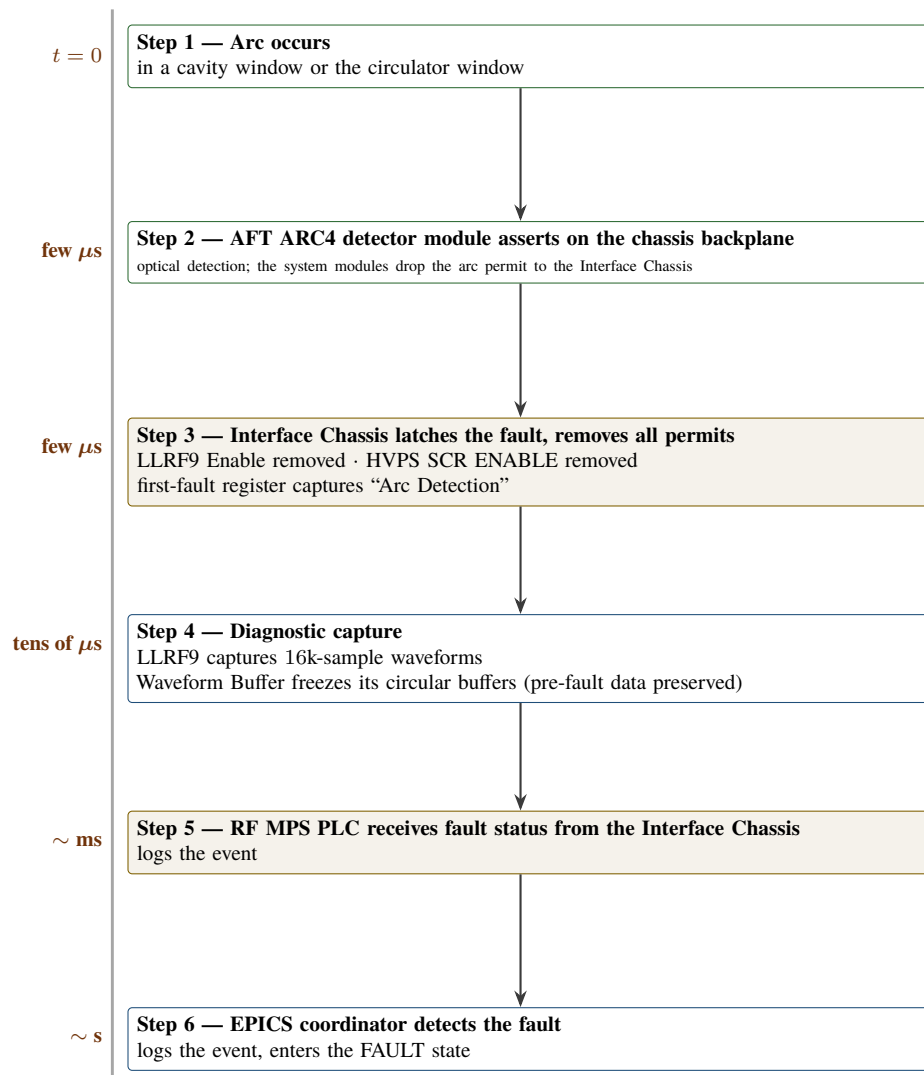
Figure 6: Fault propagation for an RF arc event. Steps 1–3 are pure hardware and complete within a few microseconds: protection is finished before any programmable device is involved. Each of the remaining steps is roughly three orders of magnitude slower than the one above it, and steps 4–6 are diagnostic and supervisory only — no protective action depends on them, so a PLC or IOC failure degrades observability but never safety.
