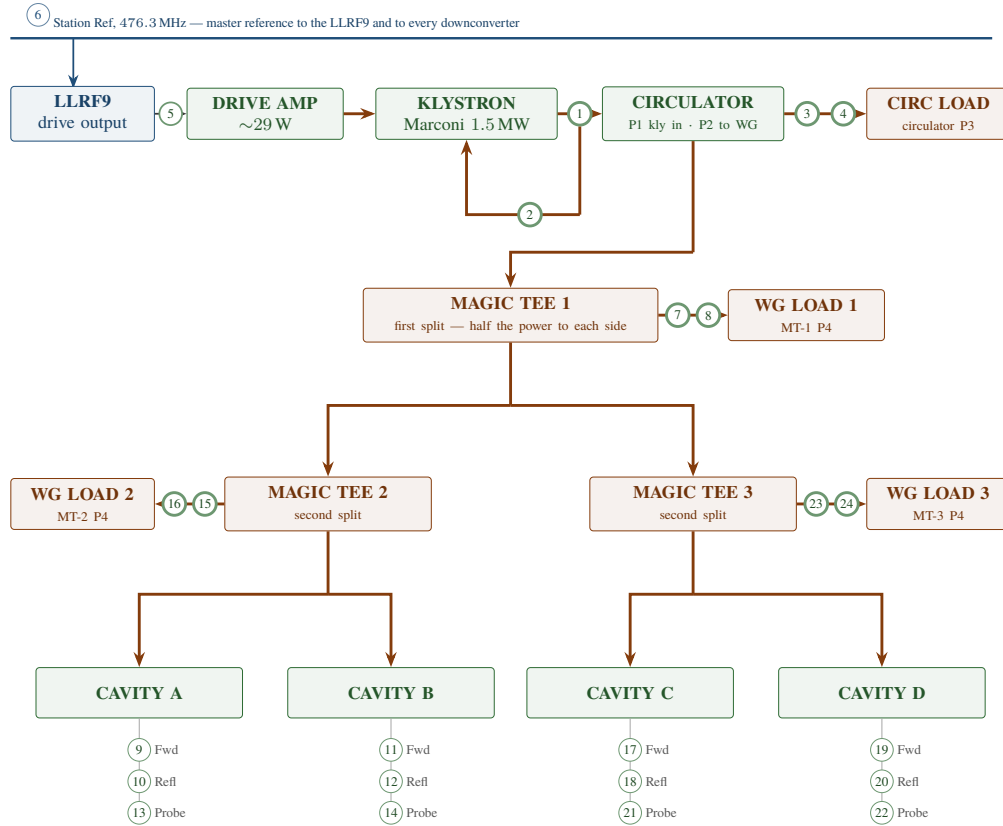
Figure 2: RF plant signal flow. Heavy lines are waveguide, light lines coaxial. Circled numbers are the directional-coupler channel indices used in §4.6. Channel 2 (klystron reflected power) branches from the bottom of channel 1 because both are ports of the same directional coupler between the klystron and the circulator.
