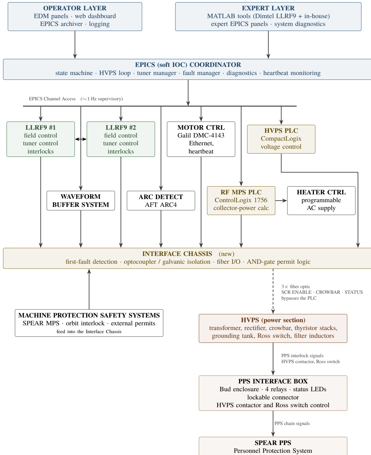
Figure 1: Upgraded system architecture. The Interface Chassis is the single hub for machine and equipment protection; personnel safety runs on a physically and logically separate path through the PPS Interface Box to the SPEAR PPS.
