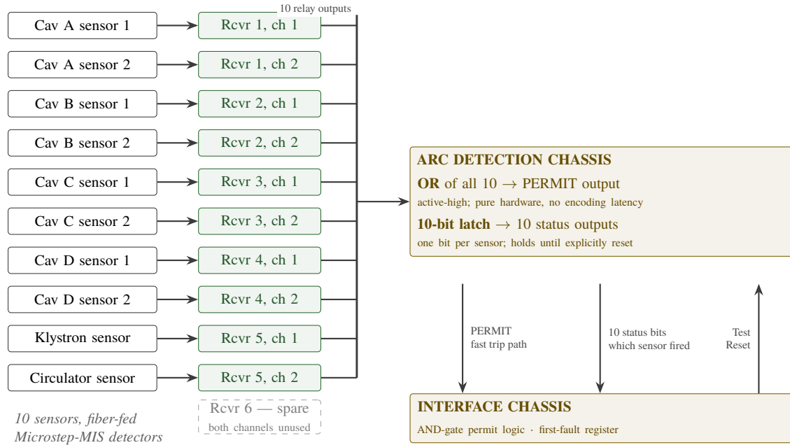
Figure 4: Arc detection signal path. The two outputs run in parallel: an all-hardware OR gives the fast trip, while the 10-bit latch preserves which sensor fired for post-mortem analysis.
