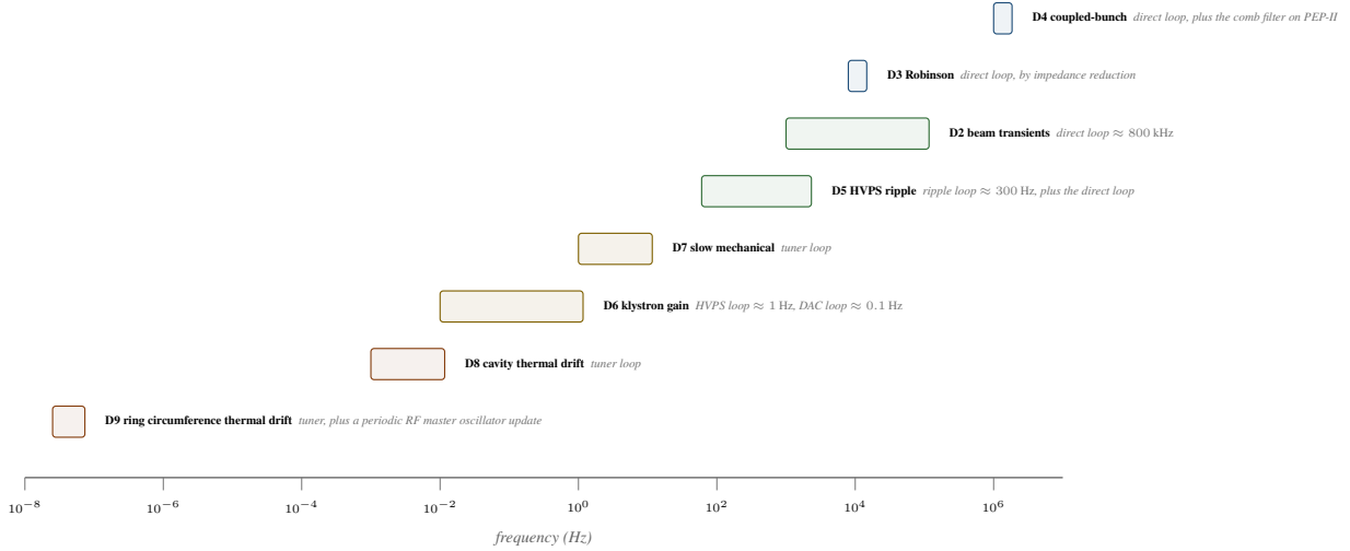
Figure 4: Disturbance spectrum and the loop assigned to each band. Loop bandwidths are separated by roughly a decade so that adjacent loops do not interact.
