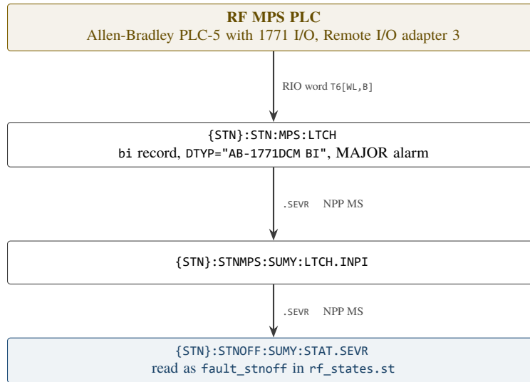
Figure 4: RF MPS PLC (Allen-Bradley PLC-5 with 1771 I/O) inputs and outputs.
