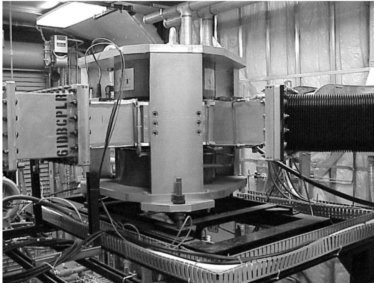
Figure 18: AFT circulator — positioned between the klystron output and the magic-tee splitter network; routes reflected power from the load network away from the klystron to protect it from reflected energy
