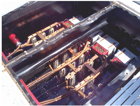
Figure 33: HVPS2 main oil tank at Building B514 — this large oil-immersed enclosure houses the phase-shift transformer (T0), the two rectifier transformers (T1, T2), the two filter inductors, four filter capacitors with their eight resistors, and the main and filter diode rectifier stacks. The SCR phase controller and the SCR crowbar are mounted inside it in their own isolated oil tanks with oil-to-oil bushings, so either can be serviced without contaminating the main tank oil [R6]. SPEAR1 is an identical installation
