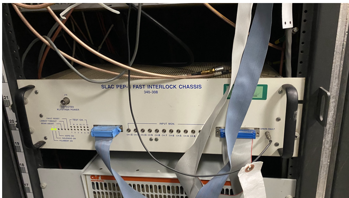
Figure 46: SLAC PEP-II Fast Interlock Chassis 340-308 in the B132: front panel showing FAULT RESET, LAMENT TIMEOUT, and BEAM ABORT controls (left cluster); 12-channel test port (TEST CH.); CH.1–CH.12 INPUT MONITOR test points (center); HVPS ON, SOLENOID ON, and FILAMENT ON status indicators; and J16 DETECTED KLYSTRON POWER coaxial input; the chassis provides sub-microsecond hardware protection by monitoring RF detector inputs and asserting SCR ENABLE removal and CROWBAR firing via fiber optic to the B514 HVPS on fault conditions
