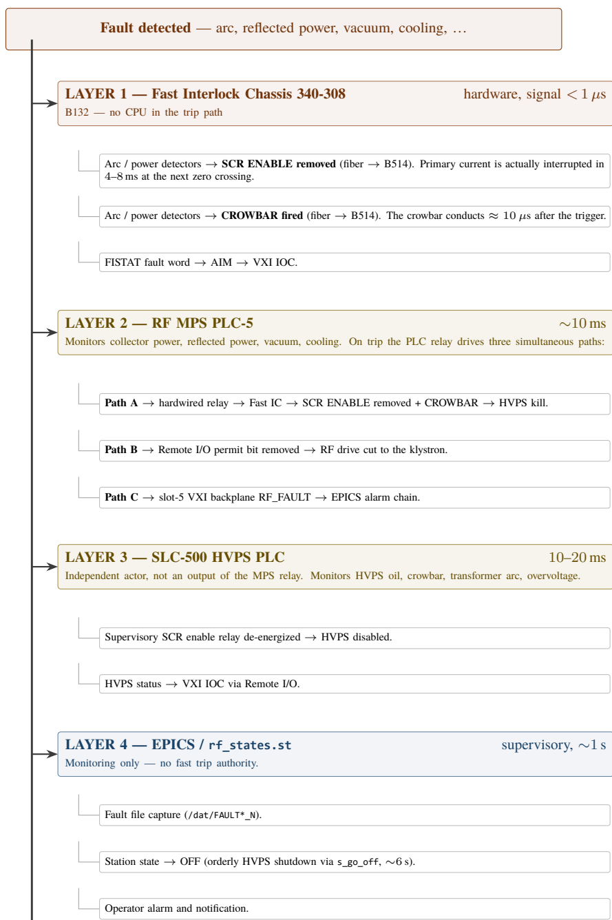
Figure 45: Complete trip chain, ordered by response time.
