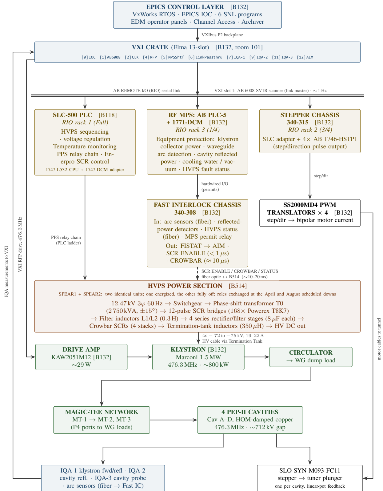
Figure 2: Top-level architecture of the legacy SPEAR3 RF station. Buildings: B132 klystron and control, B118 HVPS control, B514 HVPS power. Solid lines are electrical or hardwired connections; dashed lines are fiber optic.
