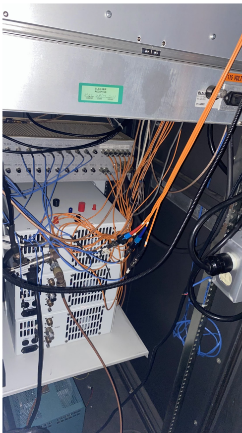
Figure 9: Rear of the LLRF VXI crate and fast interlock chassis in Building B132 — showing the dense cable plant of orange fiber optic cables (SCR ENABLE/CROWBAR/STATUS runs to B514), blue coaxial signal cables (IQA measurement inputs), and multi-conductor control wiring interconnecting the VXI modules
