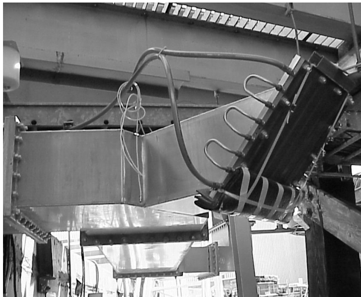
Figure 28: HOM load at an H-plane mitre bend — the three HOM loads per cavity (E-mitre, H-mitre, and plate) together damp all significant parasitic resonances above the fundamental accelerating mode
