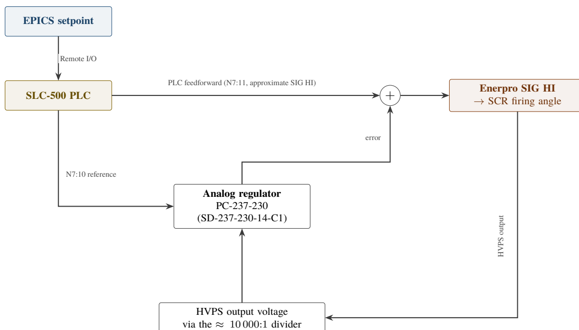
Figure 42: HVPS analog voltage regulation loop. The analog regulator card compares the PLC reference with the HVPS output voltage feedback and generates a bipolar error signal; that error is weighted and added to the PLC’s unipolar feedforward output to form SIG HI. Power-line harmonics are clearly visible on the error signal in normal operation.
