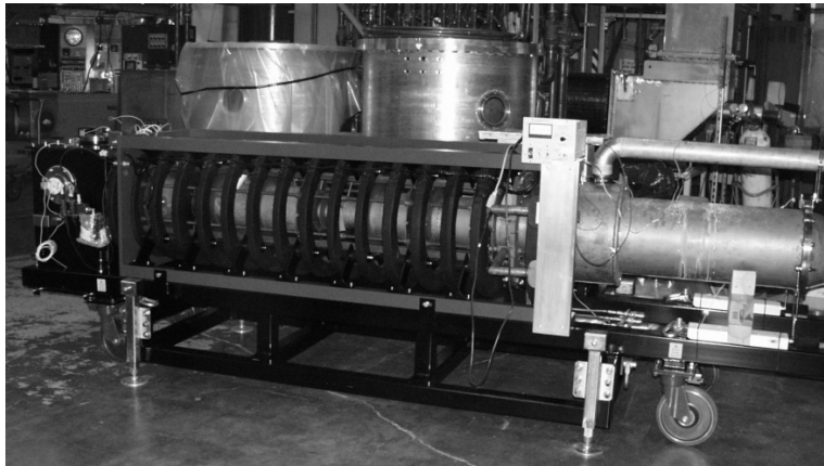
Figure 14: Marconi klystron installed in Building B132 — 476 MHz CW klystron rated ~1.5 MW, showing the collector cooling, and solenoid focusing magnets
