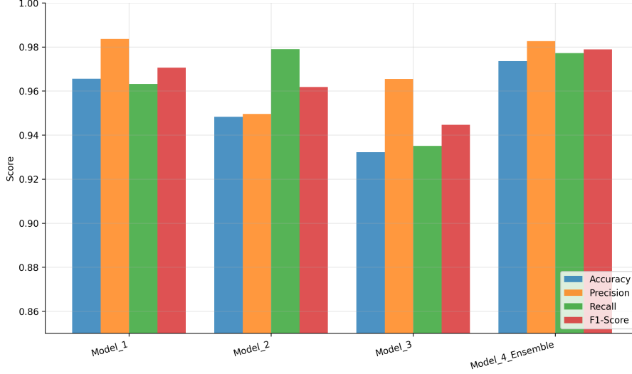
Figure 5: Model performance comparison across key metrics (Accuracy, Precision, Recall, F1-Score).
