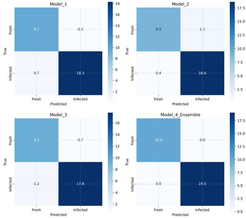
Figure 4: Confusion matrices showing mean values across 30 seeds for the four model architectures.
