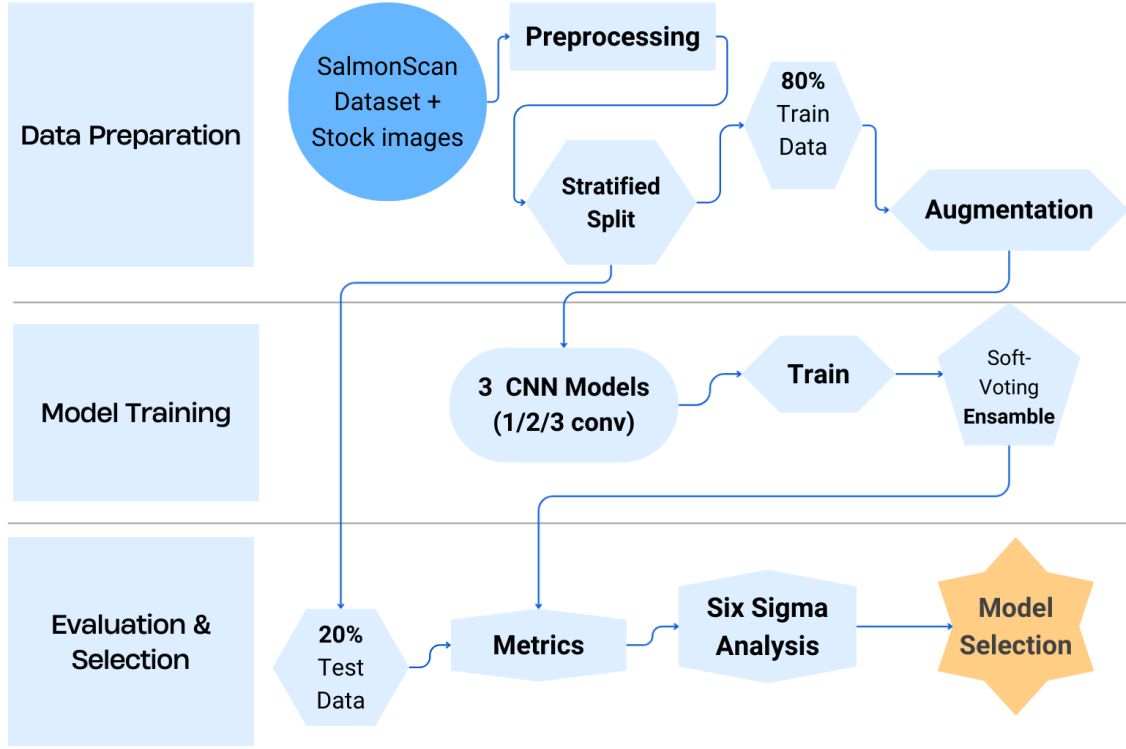
Figure 3: Methodology overview: The complete pipeline from data preparation through model selection. The SalmonScan dataset combined with stock images undergoes pre-processing and stratified splitting (80% train, 20% test), with augmentation applied to training data. Three CNN architectures with varying depths are trained and combined into a soft-voting ensemble. Final model selection is based on metrics evaluated through Six Sigma analysis.
