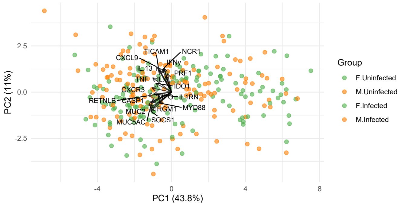
PCA Biplot: Gene Contributions to Sex/Infection Differences
