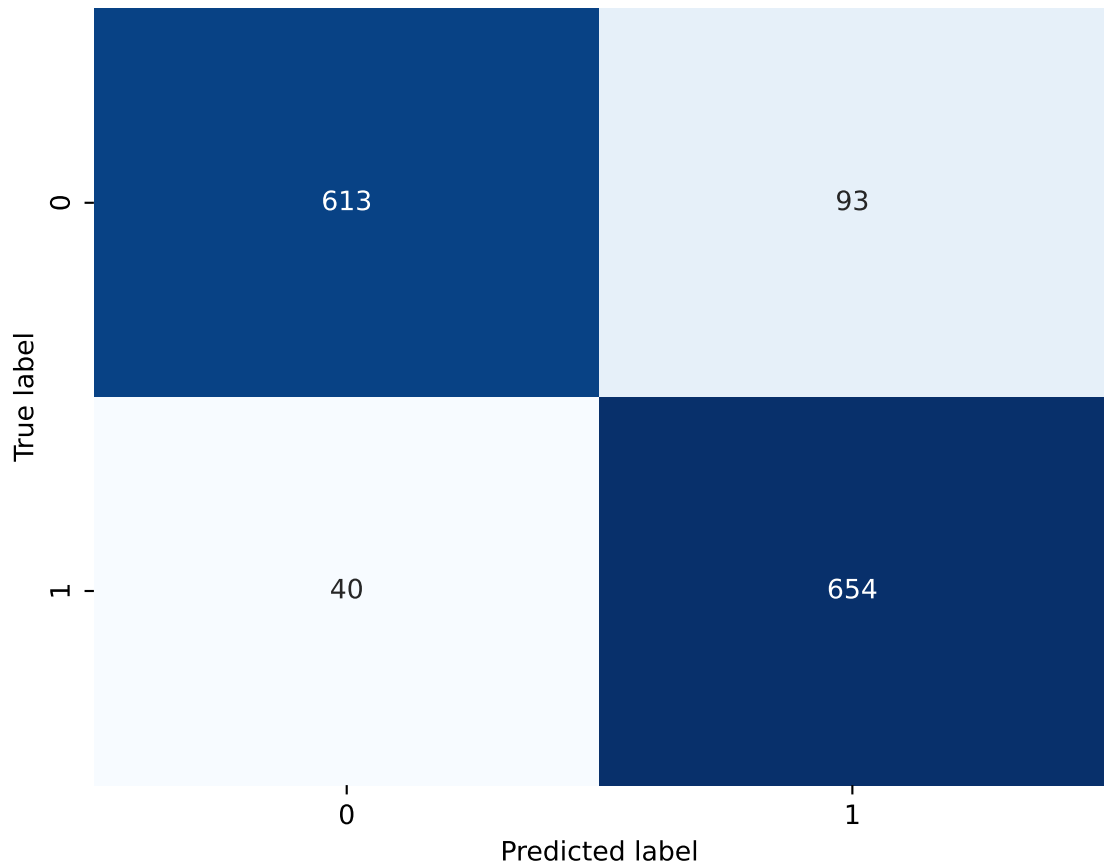
Confusion Matrix (10-fold) - GWO + SVM
