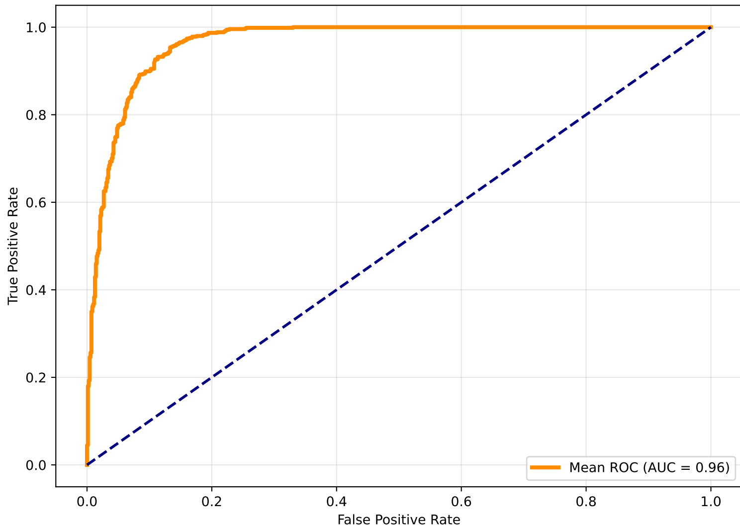
ROC Curve - GWO + SVM (10-fold)
