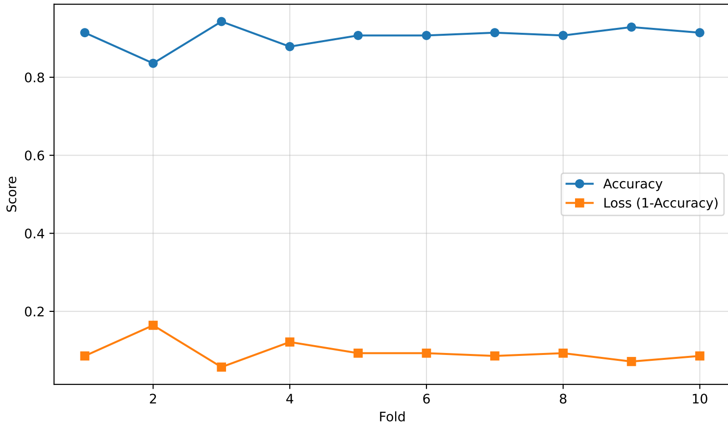
Accuracy & Loss across 10 Folds - GWO + SVM
