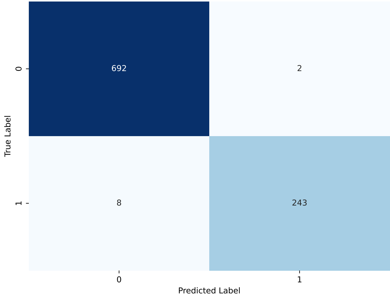
Confusion Matrix (GWO + SVM)
