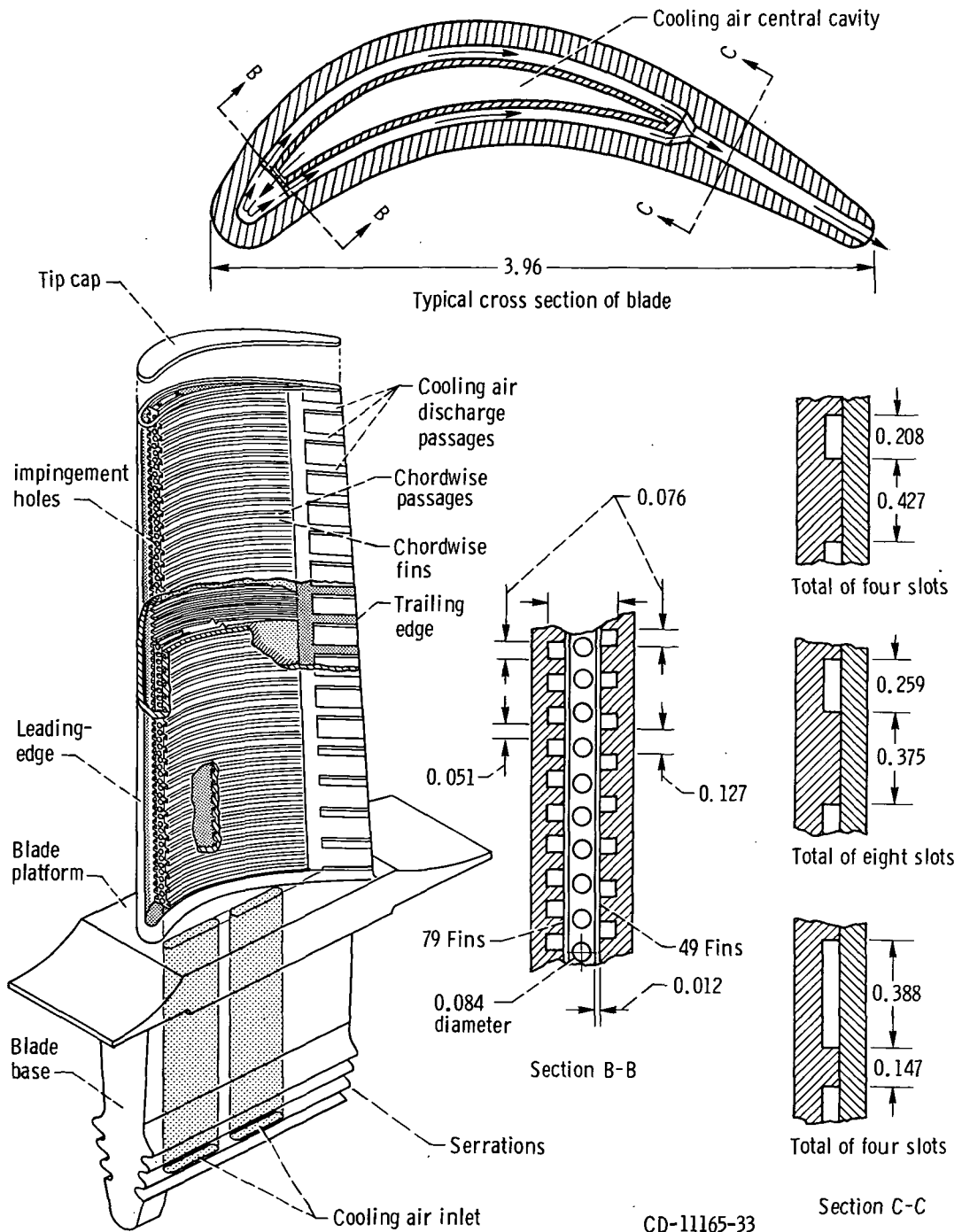
Figure 5. - Cut-away schematic of chordwise-passage air-cooled blade. (All dimensions are in centimeters.)
