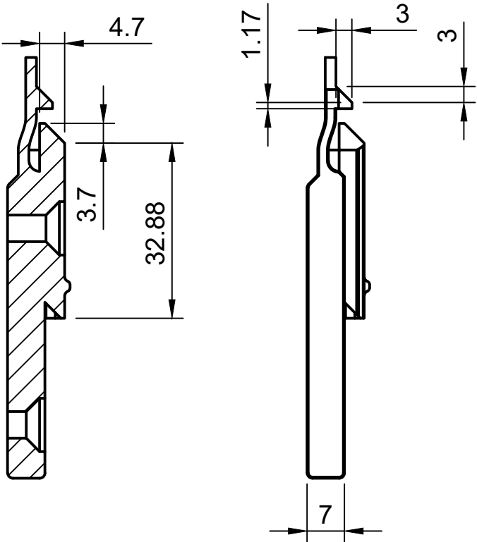
B-B (1:1)
