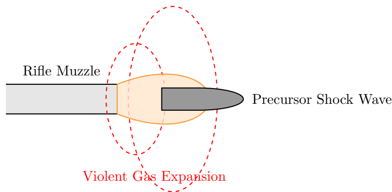
Figure 4.1: Transitional ballistics: The bullet exiting the muzzle gets overtaken by rapidly expanding, supersonic propellant gases. A symmetrical gas release here is paramount to precision (a tight group).
