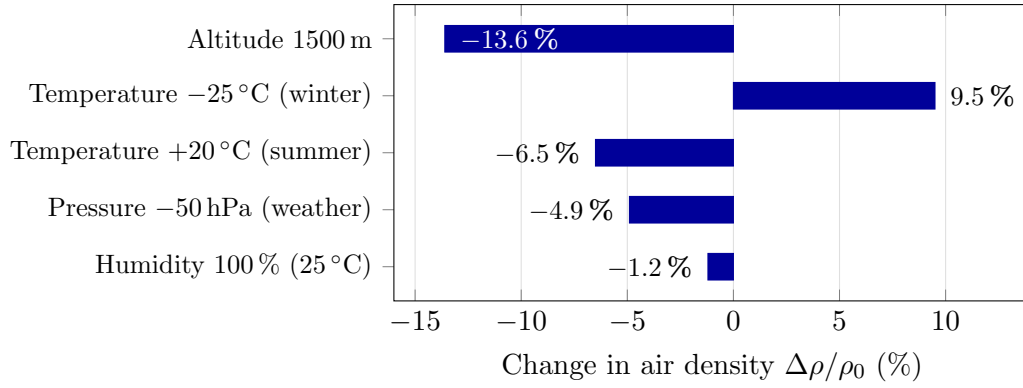
Figure 2.3: Relative change in air density for common deviations from ICAO standard conditions ( 15\text{ }^\circ\text{C} , sea level, 1013 hPa, dry air). Negative values indicate reduced density and less aerodynamic drag. Altitude and temperature are the dominant factors; humidity is negligible ( < 2\% ).
