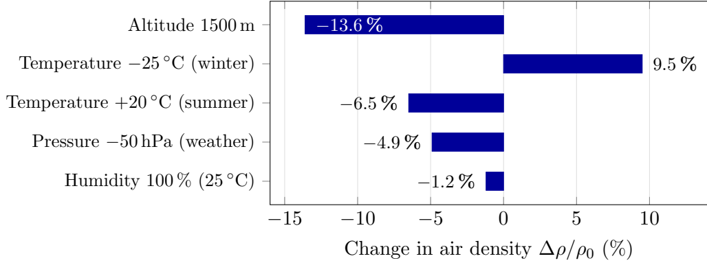
Figure 2.2: Relative change in air density for common deviations from ICAO standard conditions ( 15^\circ\text{C} , sea level, 1013 hPa, dry air). Negative values indicate reduced density and less aerodynamic drag. Altitude and temperature are the dominant factors; humidity is negligible ( < 2\% ).
